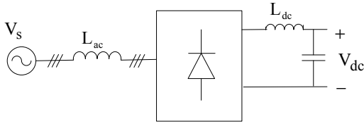
Fig. 3. AC line reactor filter ( L_{ac} ) and DC link inductance filter ( L_{dc} ).
