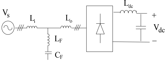
Fig. 6. Improved broadband filter.
