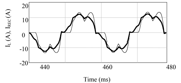
Fig. 9. Full-load line current ( I_L ) ( bold ) and rectifier current ( I_{REC} ) simulation waveforms for 5.5kW ASD system, utilizing 5 th and 7 th tuned filters.
