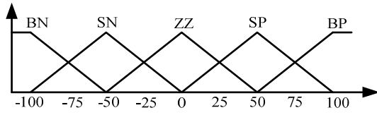
Fig.6. Membership functions of the 1st input variable ( \Delta P_{PV} ).
