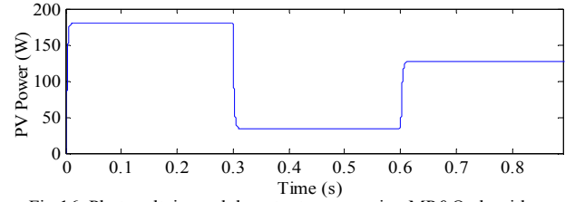
Fig.16. Photovoltaic module output power using MP&O algorithm.
