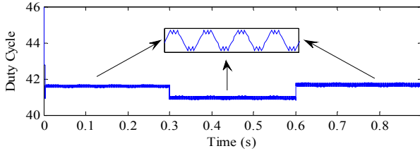
Fig.13. Duty ratio waveform of P&O algorithm.
