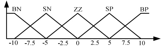
Fig.7. Membership functions of the 2nd input variable ( \Delta I_{PV} ).
