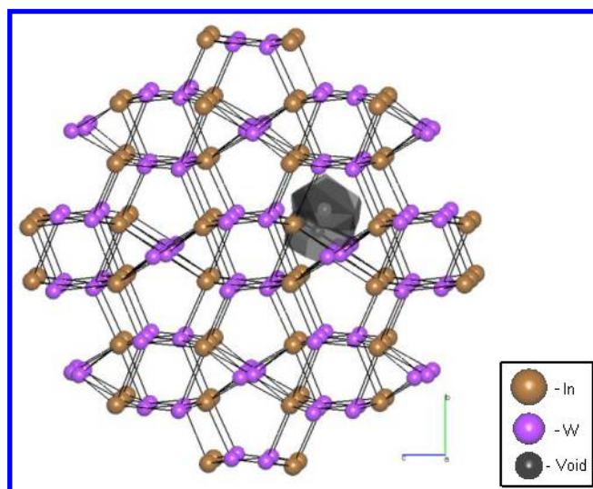
Figure 11. A representative example of a crystal structure (of \text{In}_2(\text{WO}_4)_3 [ICSD ref. 99606 – [\text{}^{119}]] ) featuring the most common ( n = 3 ) n -nodal net that bears cages with suitable void space volumes (black/grey) to contain U or Pu ions.
