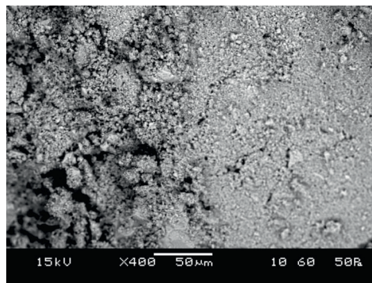
Figure 6. SEM image of sample containing Stoke Ground limestone
