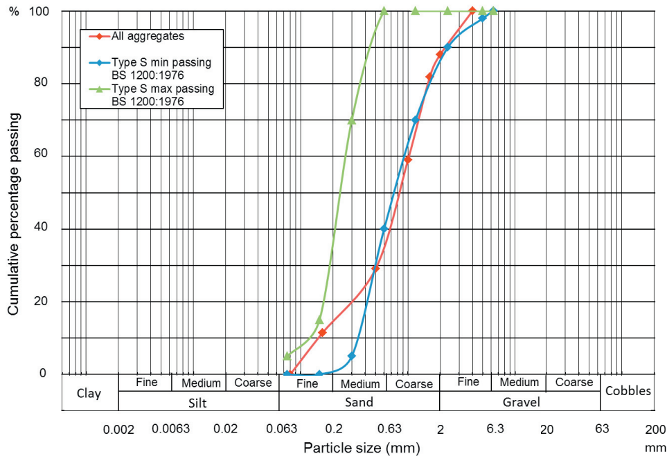
Figure 1. Particle size distribution
