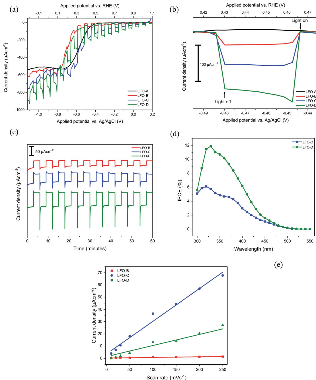
Fig. 3 (a) Current–potential curves for LFO-A, B, C, and D under chopped simulated sunlight (AM1.5G, 100 mW cm -2 ) in pH 12 0.1 M Na 2 SO 4 . Linear sweep from 0.2 to −1.12 V at 20 mV s -1 and (b) normalized current–potential measurements from (a) at point of interest (+0.42 to +0.47 V RHE ). (c) PEC stability measurements of films LFO-B, LFO-C, and LFO-D, held at +0.43 V RHE for 1 h. (d) IPCE measurements at +0.61 V RHE for LFO-C and LFO-D. (e) Current density vs. scan rate plots for films LFO-B, LFO-C, and LFO-D.
