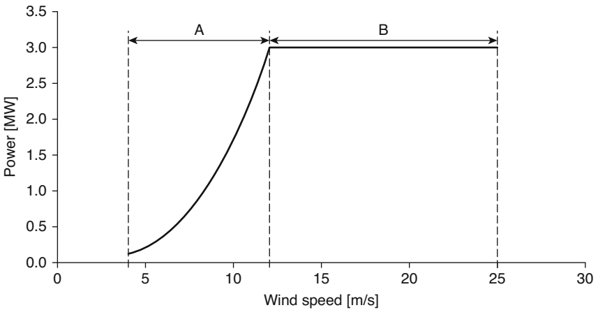
Figure 7.4 Power curve of a wind turbine
