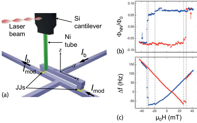
Fig. 11.15: (a) Sketch of combined torque and nanoSQUID magnetometry on a Ni nanotube. (b,c) Simultaneously measured hysteresis loops (b) \Phi_{NN}(H) , (c) \Delta f(H) . Arrows indicate H sweep direction. Dashed lines indicate discontinuities appearing in both \Phi_{NN}(H) and \Delta f(H) . (After [48] and [120])
