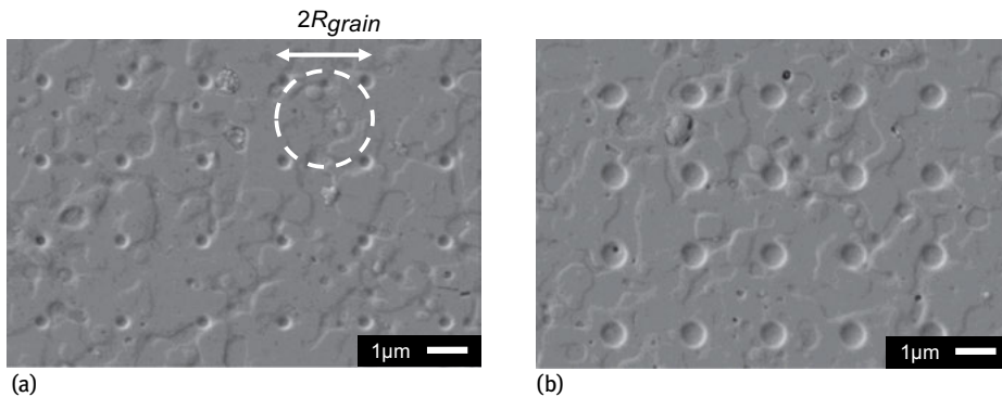
Fig. 6.8: SEM images of CSC-YBCO bridges with square patterns of circular antidots, completely perforating the film thickness, with a diameter of (a) 0.2\text{ }\mu\text{m} and (b) 0.5\text{ }\mu\text{m} . Dashed lines show an effective grain determined by the antidot pattern.
