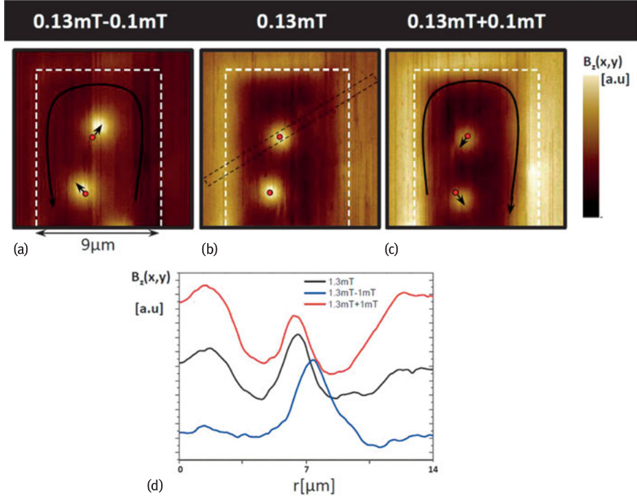
Fig. 2.5: The reaction at the end of a 9 \mu m wide superconducting Pb ribbon to a magnetic field variation is shown by making snapshots of the z-component of the local induction, B_z(x, y) , as measured by SHPM. The borders of the Pb ribbon are indicated by the dashed white line. The Pb ribbon is prepared by a field cooling procedure in a field of h_{dc} = 0.13 mT to T = 7 K (b). Two snapshots of B_z(x, y) are shown at h_{dc} = 0.23 mT (c) and h_{dc} = 0.03 mT (a) obtained upon increasing and decreasing the field with 0.1 mT after preparing the ribbon as described. In (d), the average cross section is shown for the different field configurations, as obtained by averaging the cross sections in the rectangular area indicated by the black dashed line in (b).
