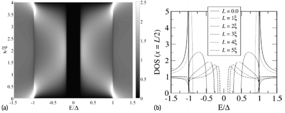
Fig. 3.13: (a) LDOS within the portion N of an SNS junction of a diffusive N bridge of length L = 4\xi calculated in the framework of Usadel theory. Note the appearance of a constant width minigap through N. (b) LDOS in the middle of an SNS junction as a function of energy for different lengths of the wire N, L = 0 - 5\xi [18].
