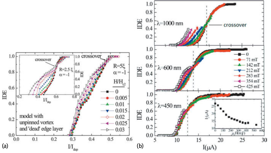
Fig. 9.3: SSPD IDE dependence on the bias current normalized to the depairing current at different magnetic field values [37]. (a) Hot spot model calculations with the radius R_{\text{spot}} = 5\xi . The inset shows the same case but with R_{\text{spot}} = 2.5\xi . (b) Experimental results for an NbN SSPD operated at three different wavelengths (photon energies). Curves corresponding to the strongest fields can be broken before reaching the expected crossover current due to the critical current limitation, see the inset.
