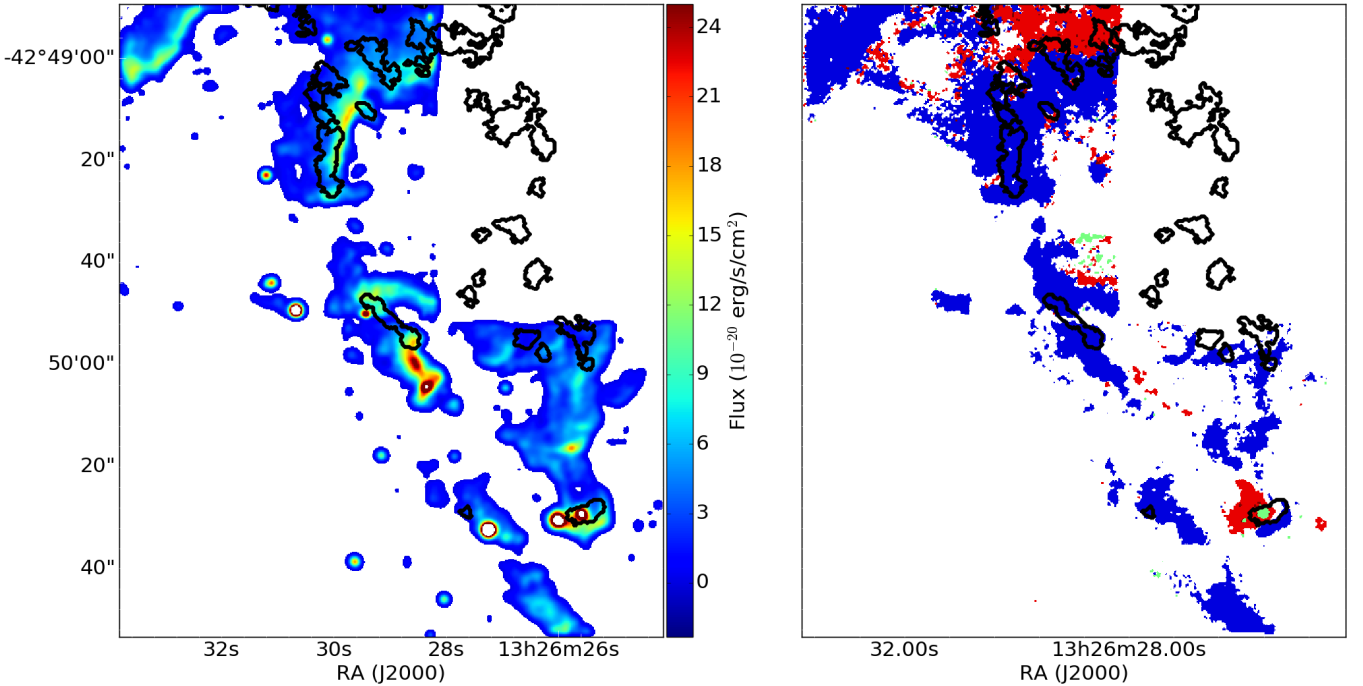
Fig. 8: Maps of the \text{H}\alpha -[NII] flux from MUSE (left) and the excitation processes of the CO structures (right). The black contours represent the ALMA CO(1-0) emission distribution. The BPT diagram was computed for the velocity range -330 < v < -120 \text{ km.s}^{-1} . Star formation is represented in green and AGN or shocks are indicated in blue. Red corresponds to a composite of star formation and AGN/shocks. The CO clouds in the Horseshoe complex are associated with shock-excited \text{H}\alpha emission, except for one clump that is associated with the star-forming region from Santoro et al. (2016) and young stellar clusters.
