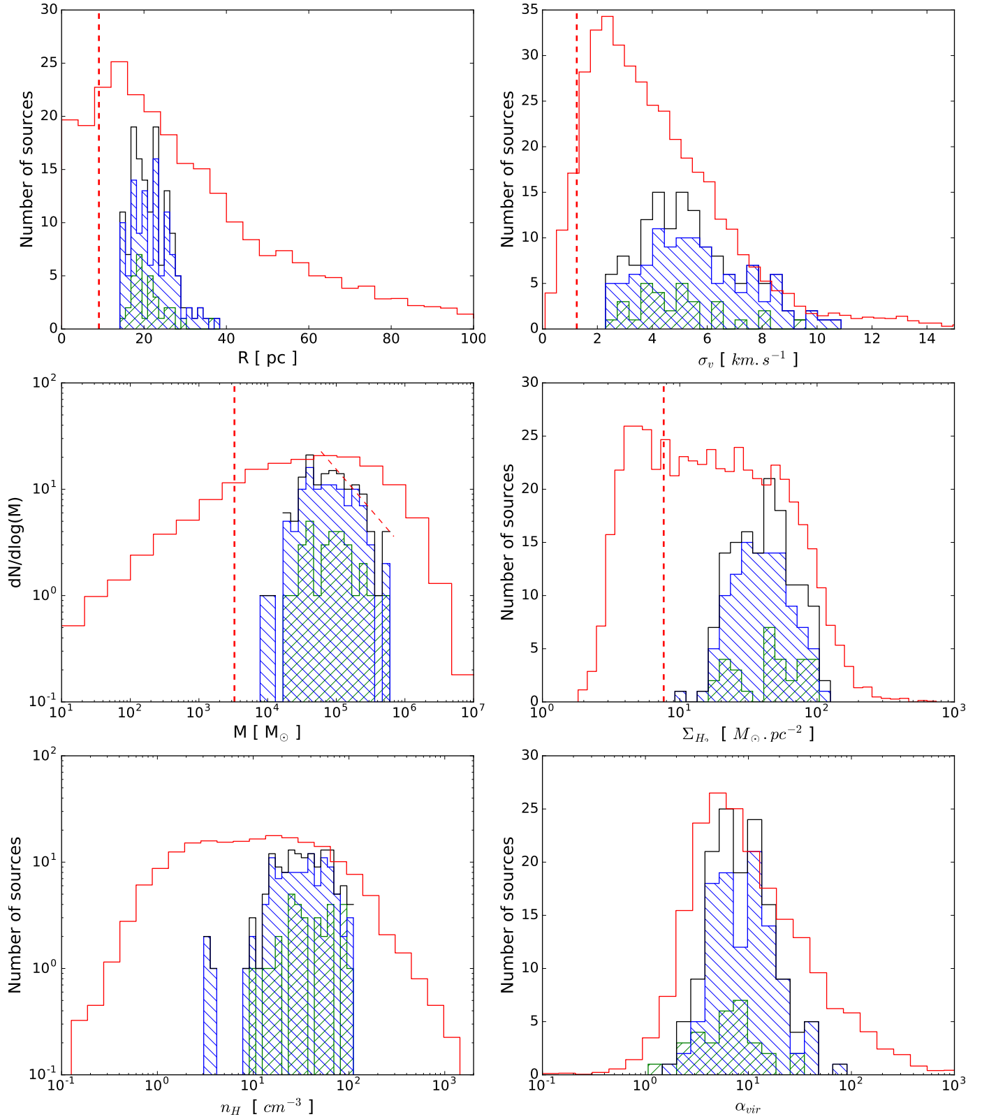
Fig. 3: Histogram of the properties of the giant molecular clouds. Top : Characteristic radius and velocity dispersion. Middle : Molecular gas mass and surface density. The red dashed line in the left plot is the best fitting power law for masses M \geq 9 \times 10^4 M_\odot . Bottom : Volume density and virial parameter. The vertical red dashed lines correspond to the lower limits due to resolution or sensitivity. In the six plots, we added the histograms of GMCs of the Milky Way (Miville-Deschênes et al. 2017). The clouds were separated in two groups: (i) the Horseshoe complex in blue, where gas is excited by shocks; and (ii) the star-forming clouds in green, associated with H\alpha , FUV emission, and young stellar clusters.
