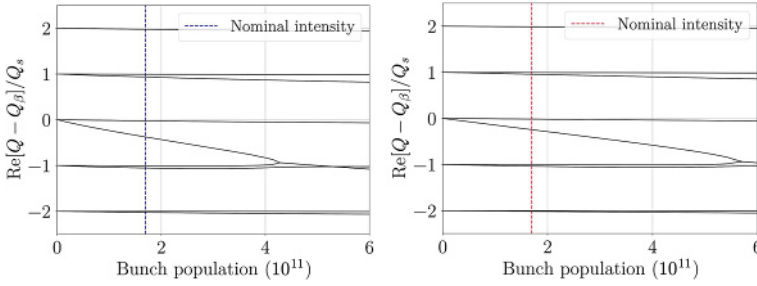
Fig. 2.31. Real part of the frequency shift of the first coherent oscillation modes as a function of the bunch population without (left) and with (right) beamstrahlung, by considering only the RW impedance produced by a NEG film with 100 nm thickness.
