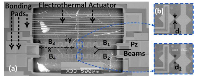
Fig. 3. SEM image of the prototype microchip, (a) meander-shape beams ( B_1, B_2, B_3, B_4 ), electrothermal actuator ( x=850\mu\text{m} , y=100\mu\text{m} ), (b) magnified image of shuttle protrusions and beam tips ( d_1=5\mu\text{m} , d_2=10\mu\text{m} ).
