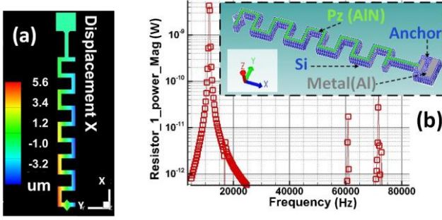
Fig. 4 Finite element analysis, (a) tip displacement in X direction in response to the force in Y direction that pluck the beam, (b) Harmonic balance analysis, the spectrum of power delivered to a 1MΩ resistor.
