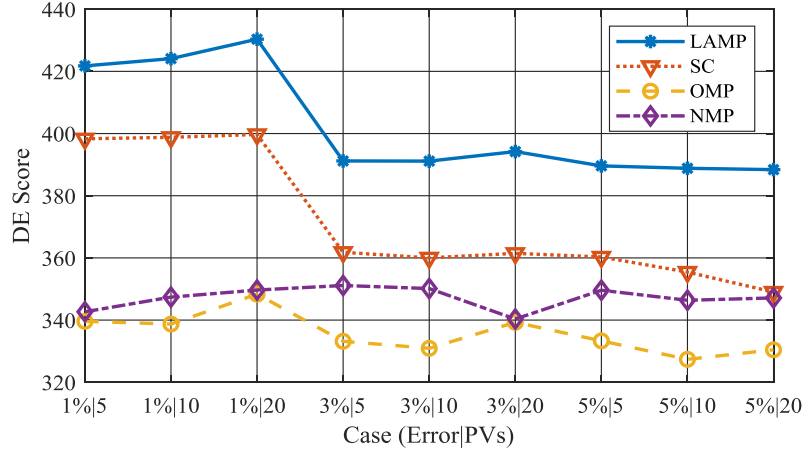
Fig. 16 The scores of LAMP, SC, OMP and NMP algorithms under different forecasting errors and PV numbers with 50 EVs.
