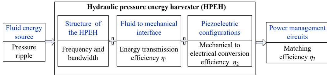
Figure 3. Factors related to the energy harvesting performance of hydraulic pressure energy harvesters.
