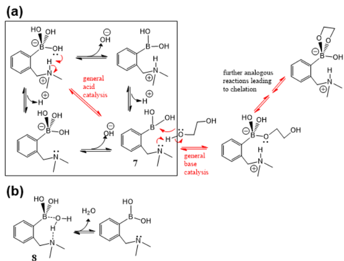
Figure 4. Mechanistic considerations for the role of the o -aminomethyl group. (a) The proposed mechanism for boronate ester formation at pH's between the first and second pK a 's, based upon kinetics, crystal structures, and isotope effects. The red equilibrium arrows show the dominant pathway, involving general acid-catalyzed expulsion of an inserted solvent with a general base-catalyzed delivery of the guest. (b) The possibility of losing the inserted solvent in a single step if the solvent is not highly ionized between the N and B.
