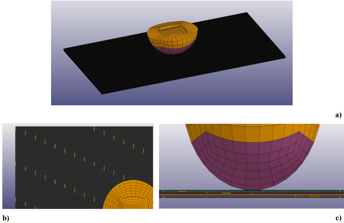
Figure 15- FEA model layout for LVI test: a) isometric view, b) top view and c) lateral view.
