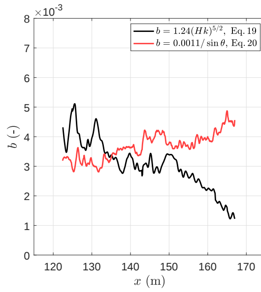
Figure 8. Cross-shore evolution of the dissipation coefficient b (Eq. 17), computed with the wave group ensemble-averaged data (same wave group as Figure 5) using the formulation of D81 (Eq. 20) and that found later by Drazen et al. [2008] (Eq. 19).
