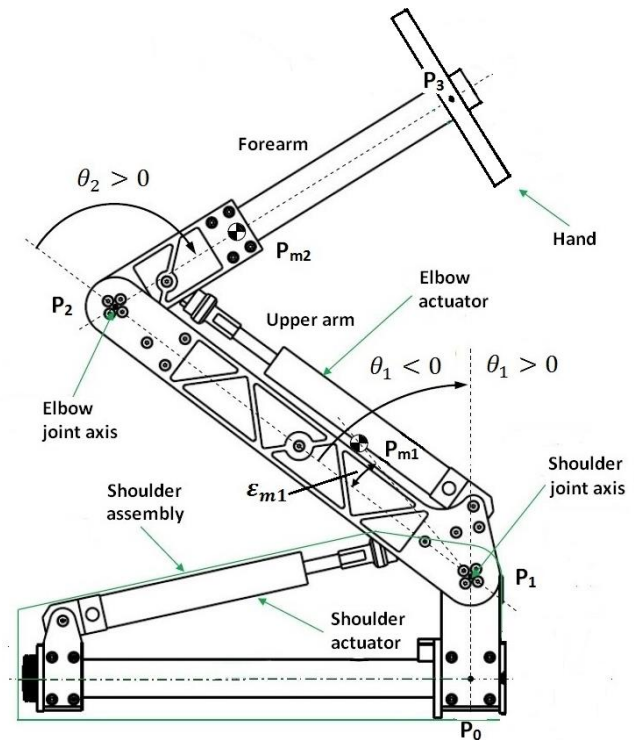
Figure 12 Geometry of the robot arm (modified from [19])
