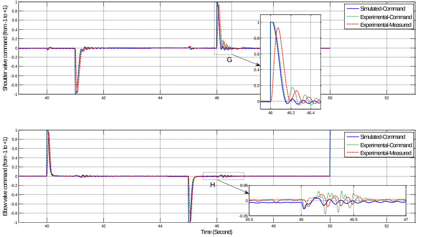
Figure 14 FPVC square wave responses – commanded and actual valve spool positions
