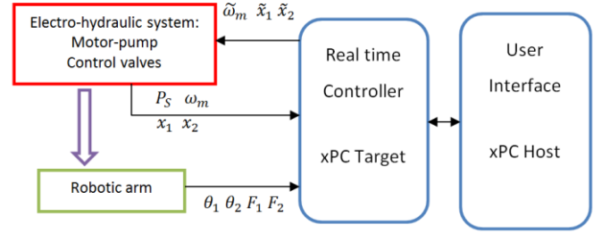
Figure 11 Test rig control architecture
