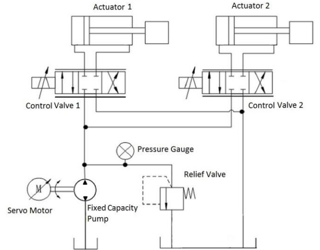
Figure 1 The hydraulic circuit diagram of a plant with two actuators
