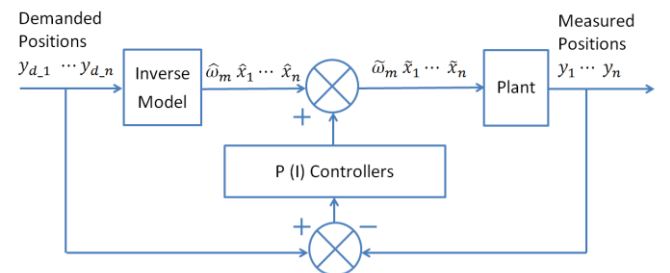
Figure 2 The VPVC control algorithm
