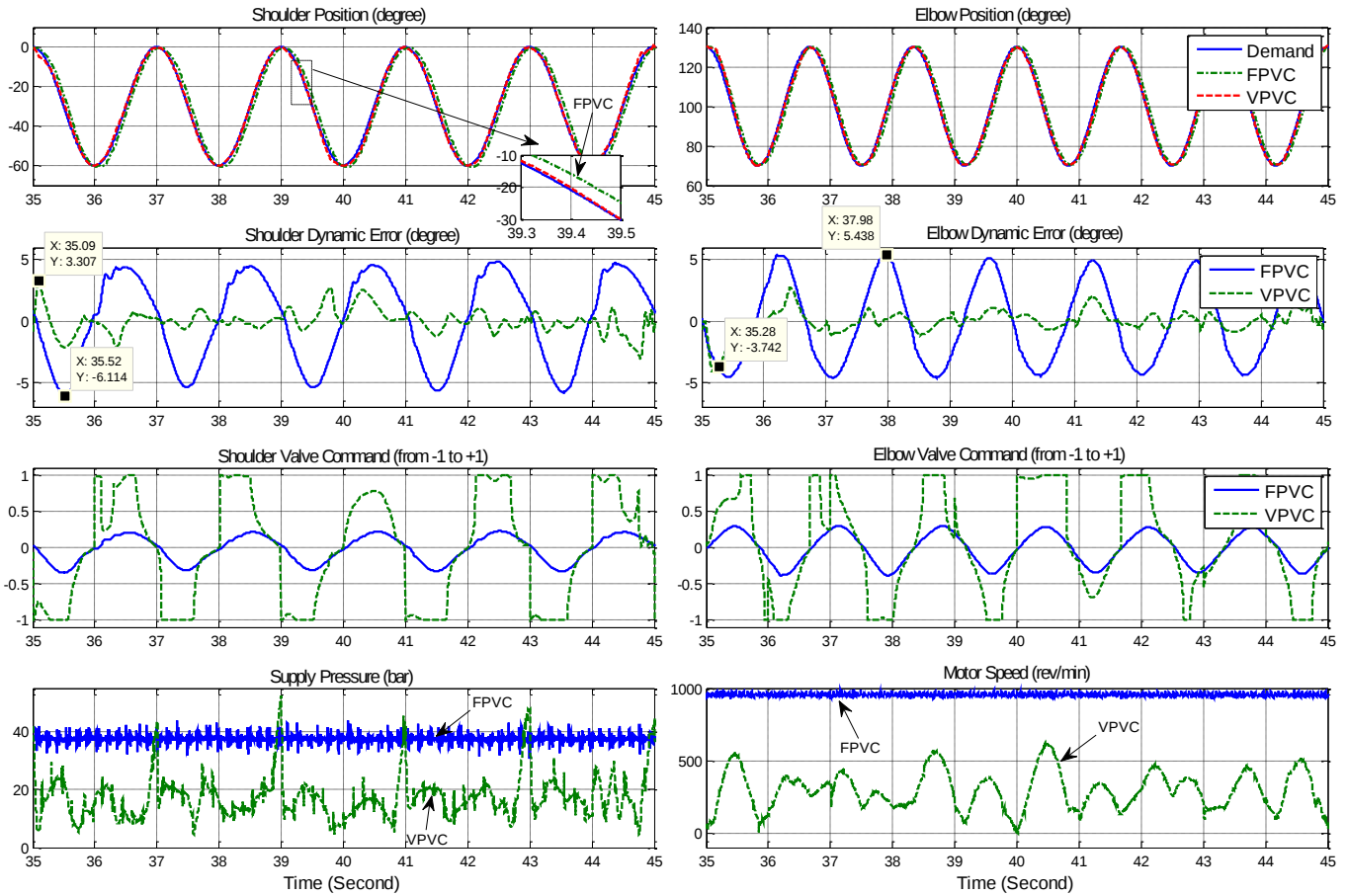
Figure 18 Experimental FPVC and VPVC comparison (Test 3)
