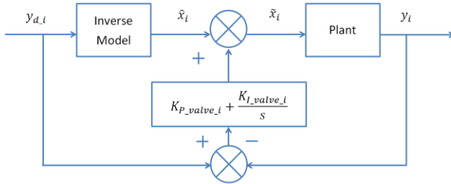
Figure 7 VPVC valve command adjustment
