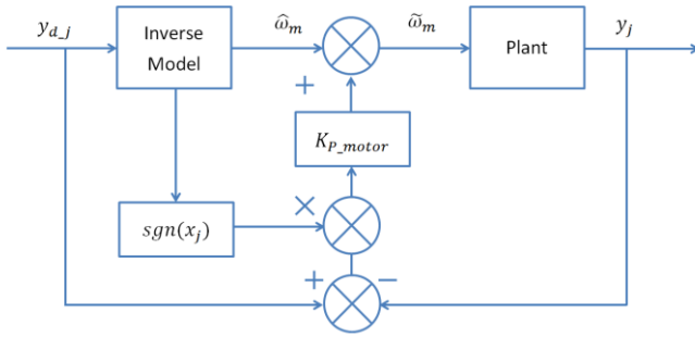
Figure 6 VPVC motor speed command adjustment
