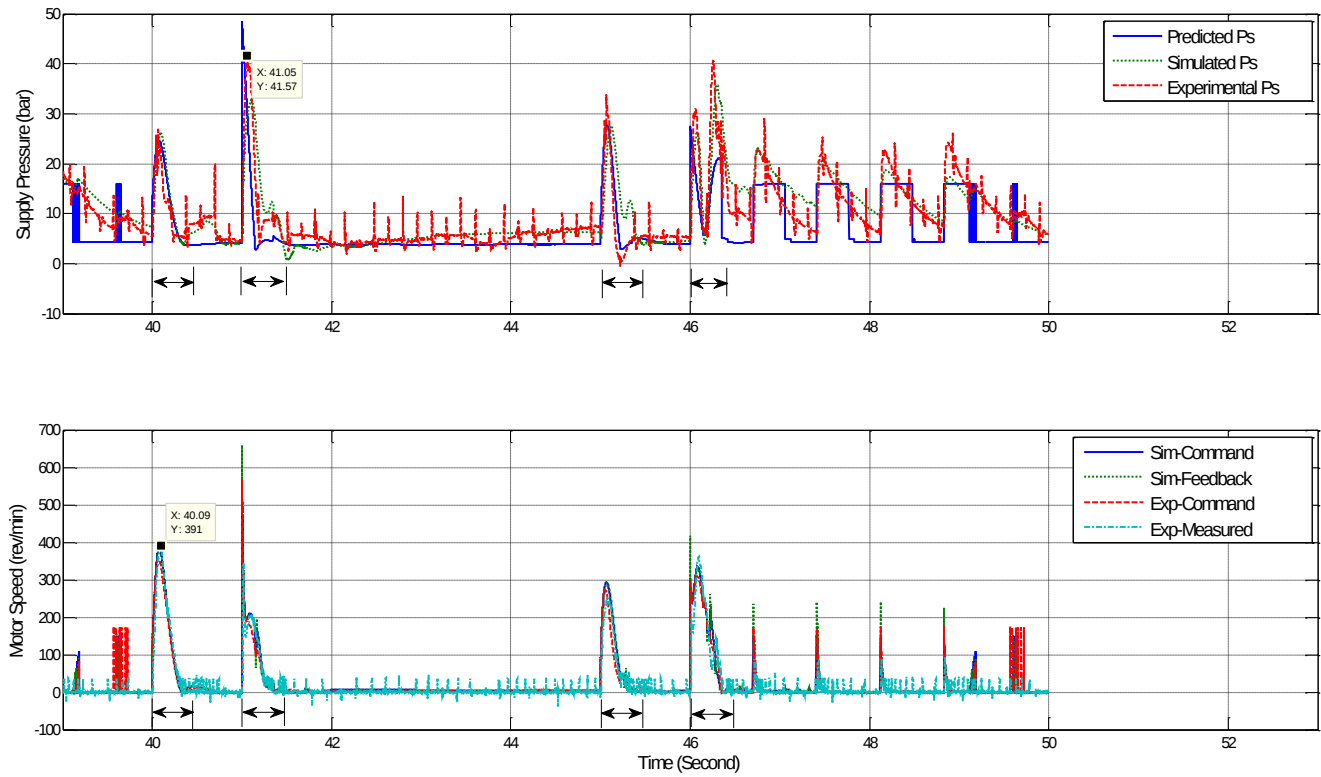
Figure 17 VPVC filtered square wave responses– supply pressure and motor speed
