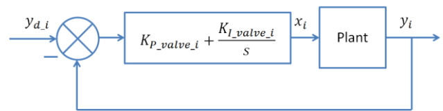
Figure 8 Proportional-integral control of FPVC system
