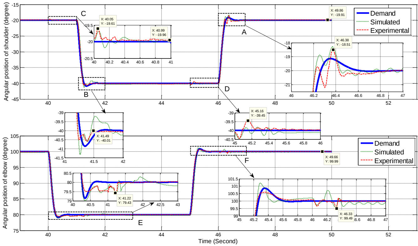
Figure 15 VPVC filtered square wave responses – demand and actual joint positions
