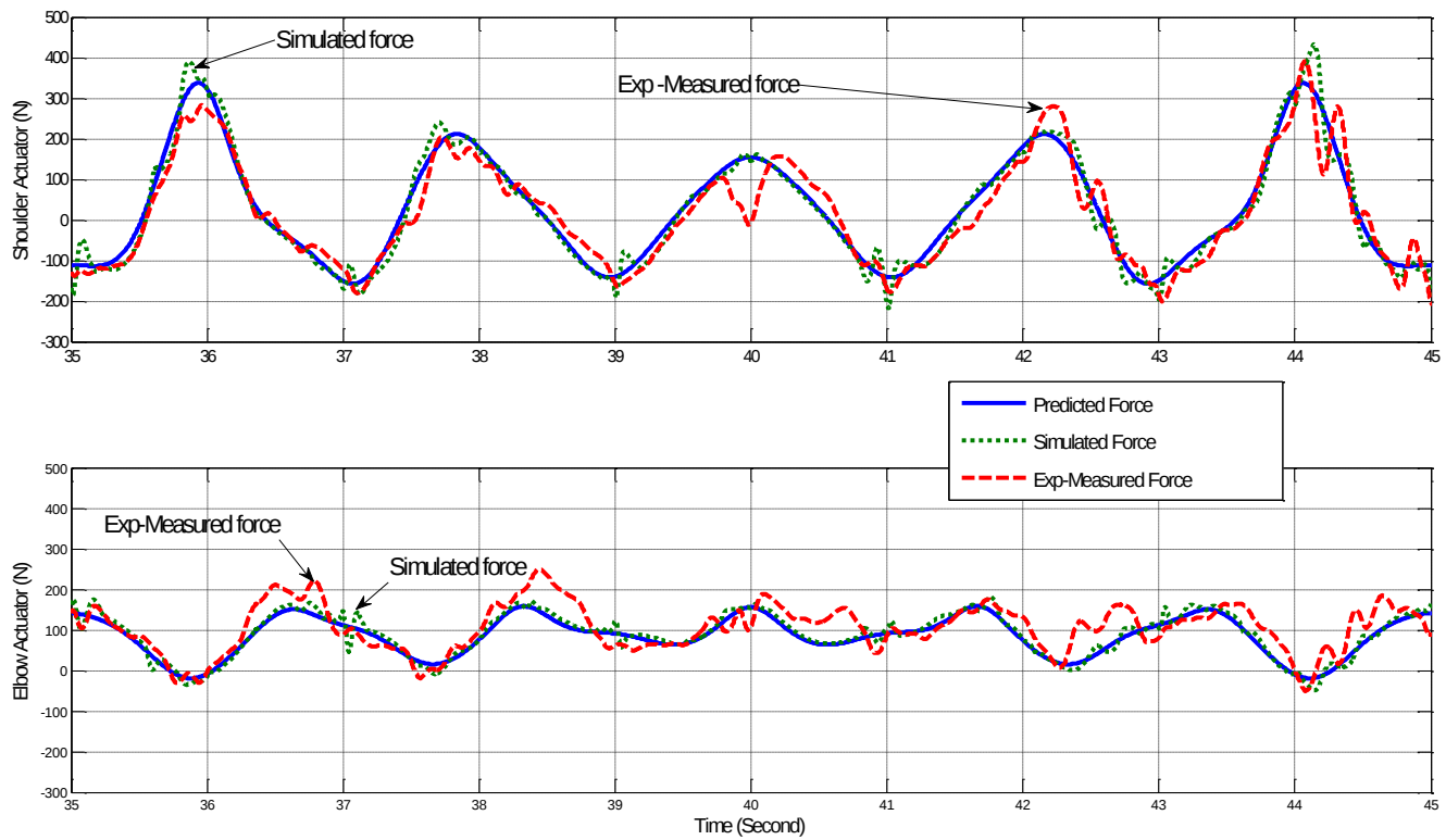
Figure 19 VPVC actuation force (Test 3)
