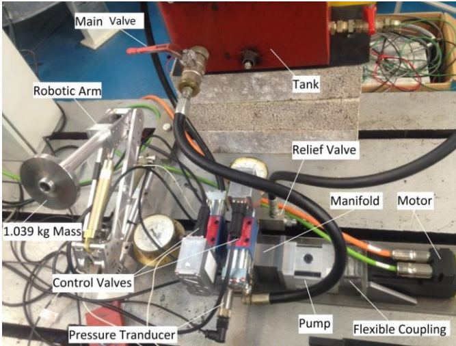
Figure 10 Electrohydraulic components
