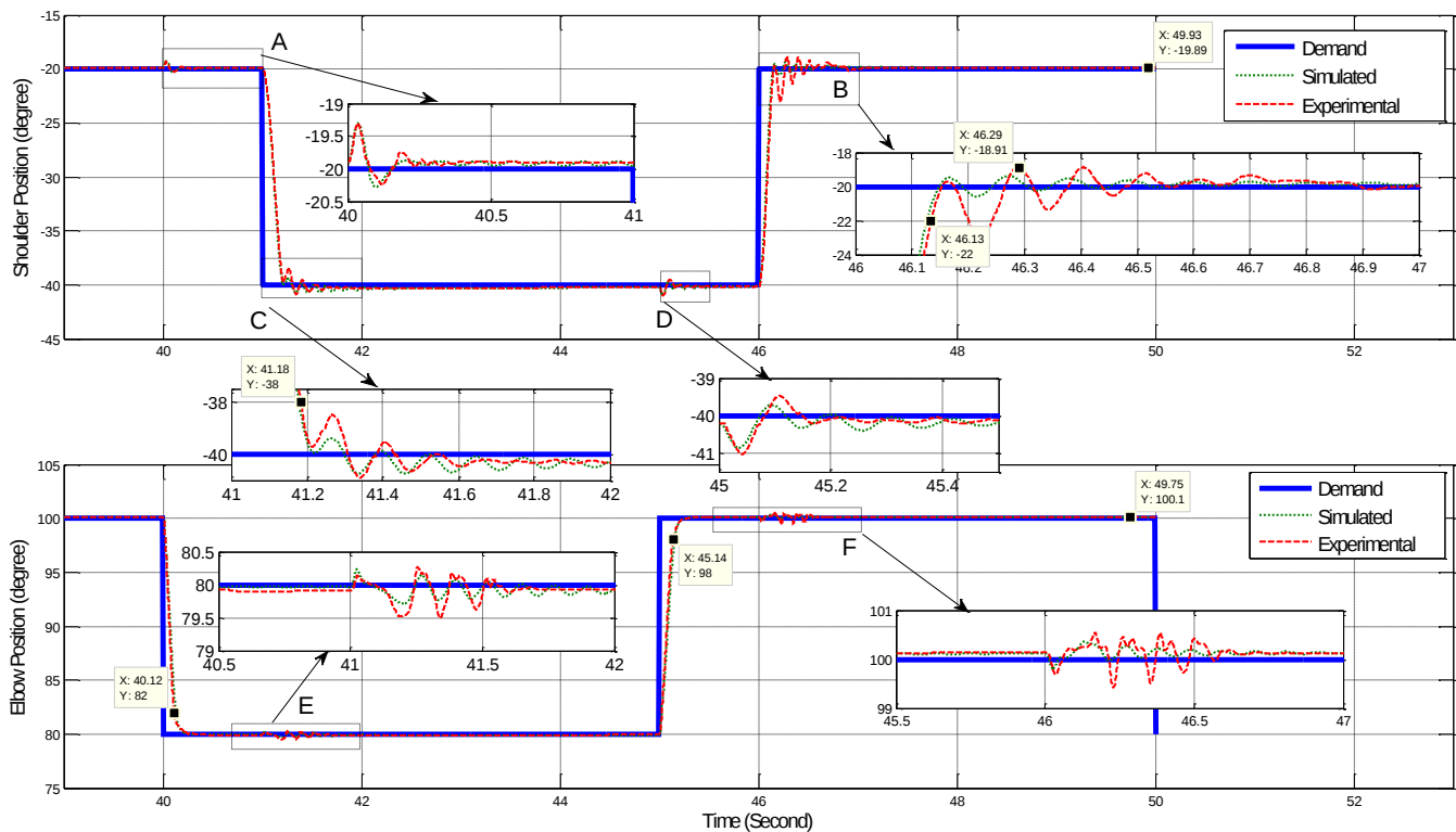
Figure 13 FPVC square wave responses – demand and actual joint positions
