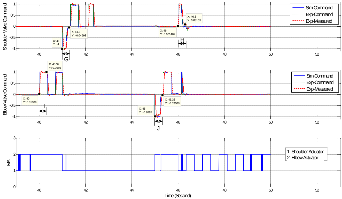
Figure 16 VPVC filtered square wave responses – commanded and actual valve spool positions
