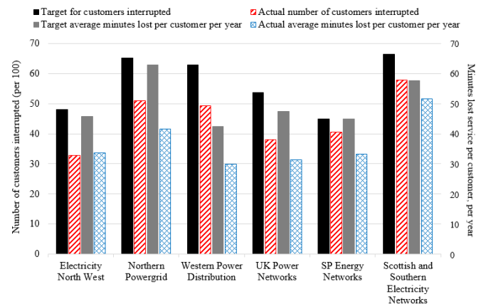
Figure 1. UK Customer interruptions and minutes lost 2016-17 [4].
