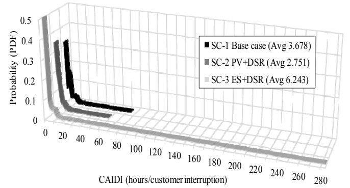
Figure 2. Impact on the duration of interruptions to affected customers.
