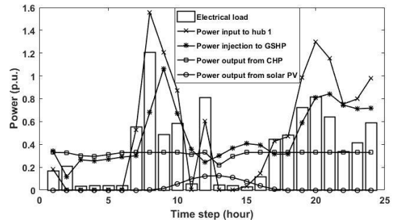
Fig. 10. Optimal strategy of hub 1 over 24 hours
