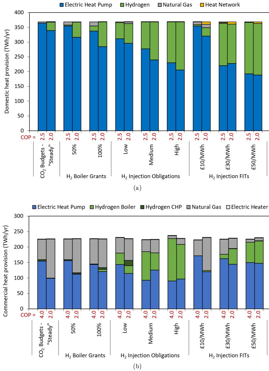
Figure 4: Heating provision in (a) the domestic sector and (b) the commercial sector in 2050-2060 for a range of scenarios, comparing the original COPs with the sensitivity scenarios with COP = 2.
