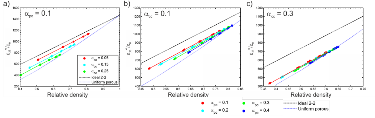
Figure 8: Variation of relative permittivity \varepsilon_{33}^{\sigma}/\varepsilon_0 with relative density for a) varying ceramic channel porosity \alpha_{cc} , \alpha_{pc} = 0.1 , b) varying ceramic fraction in pore channel \alpha_{pc} , \alpha_{cc} = 0.1 , and c) varying ceramic fraction in pore channel \alpha_{pc} , \alpha_{cc} = 0.3 . The relative permittivity for an ideal 2-2 structure ( \alpha_{cc} , \alpha_{pc} = 0 ) and uniformly distributed porous barium titanate as a function of relative density are shown for comparison (black and violet dashed lines, respectively) in all figures.
