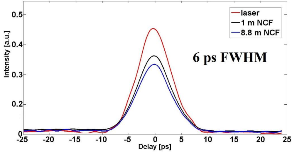
Fig. 9. Intensity autocorrelation traces of: picosecond laser light (35 \mu J, solid red line); transmitted beam through 1m fiber (30 \mu J, solid black line) and 8.8 m NCF (21.5 \mu J, solid blue line).
