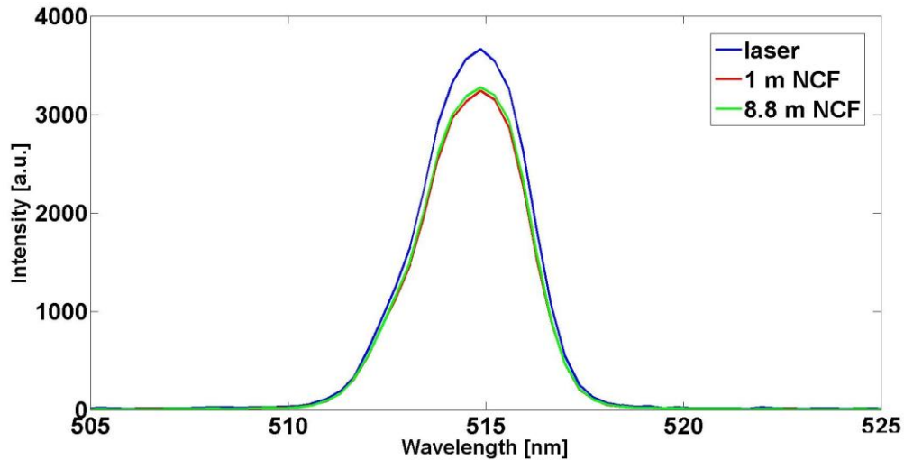
Fig. 8. Optical spectra of: picosecond laser beam (35 \mu\text{J} pulse energy, solid blue line); delivered beam through 1 m NCF (30 \mu\text{J} pulse energy, solid red line) and 8.8 m NCF (21.5 \mu\text{J} pulse energy, solid green line).
