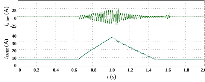
Fig. 18. Experiment waveforms of phase-A inverter current and SMES current.
