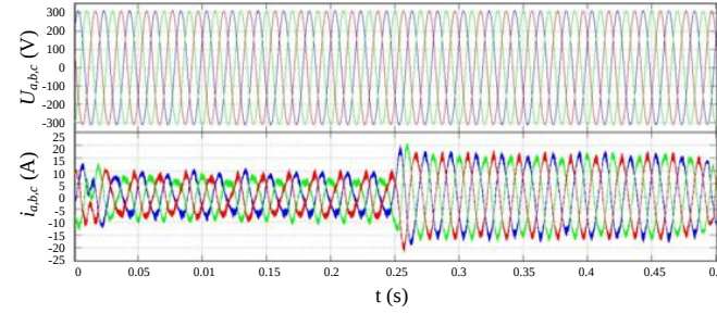
(b) 3-phase voltage and current simulation waveforms in discharging mode
