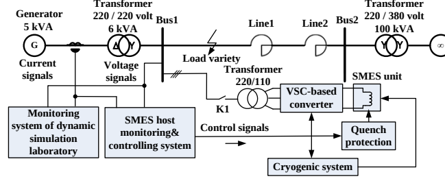
Fig. 15. Circuit diagram of the power compensation experiment.
