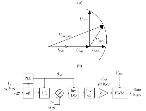
Figure 2. Vector diagram of DVR control strategies [1] U_{drv1} : 'In phase compensation'. U_{drv2} : 'Pre-sag compensation'. U_{drv3} : 'Energy optimal control'. (b) DVR control system.
