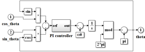
Figure 3. Simulink implementation of PLL algorithm where \omega_0 is the fundamental output frequency in rad/s.
