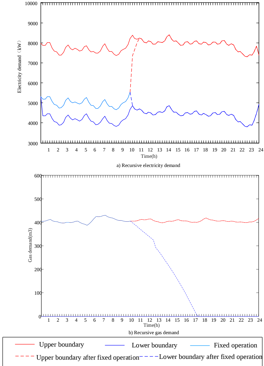
Fig 18 Recursion of ACI
