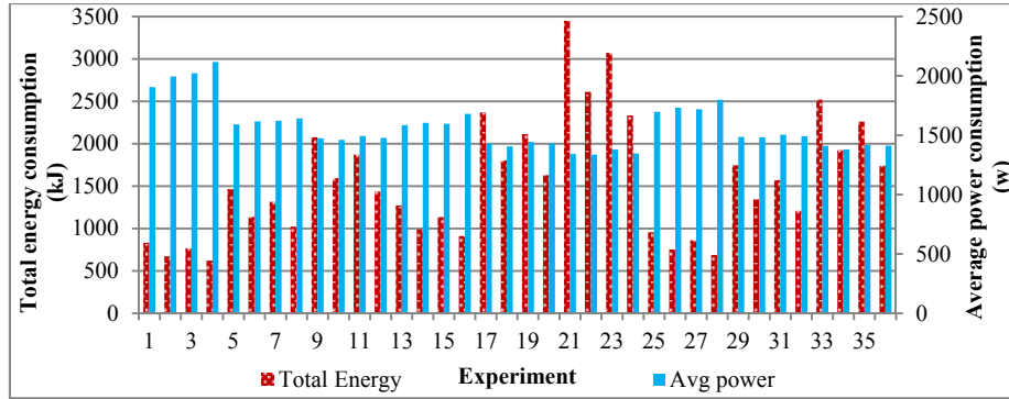
Fig. 3. Energy consumption and power consumption graphs of the experiments
