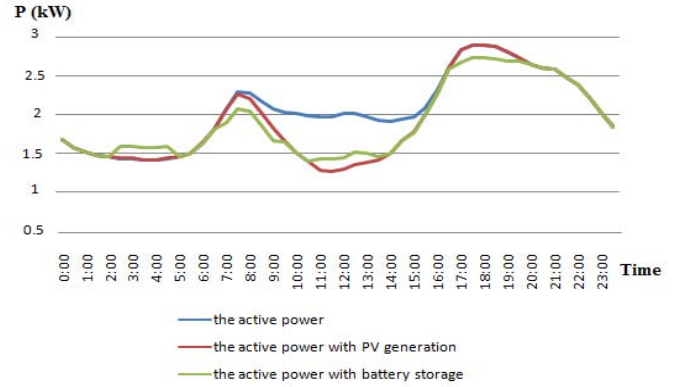
Fig.10 the active power with and without battery storage per household
