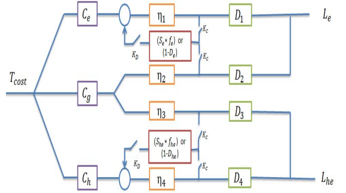
Fig. 4. SDF control energy hub modeling overview
