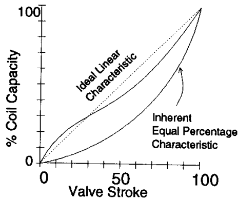
Figure 12: Shift of Equal Percentage Characteristic Due to Changing \Delta P at Valve
