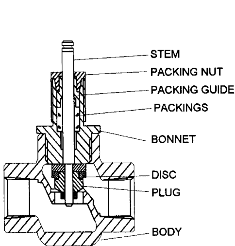
Figure 1: N.O. VT Valve Body
