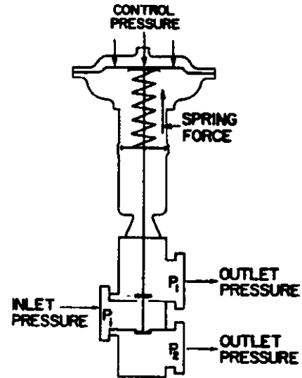
Figure 17: Three-Way Bypass Valve
