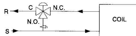
Figure 18b: Mixing Valve in a Bypass Application Piped NC. to Coil
