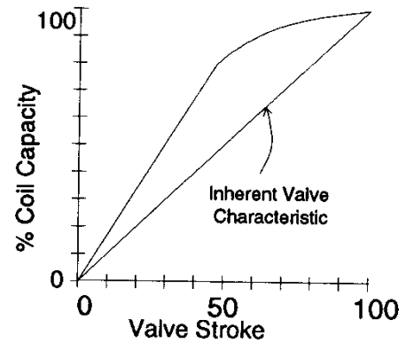
Figure 13: Shift of Linear Valve Characteristic Due to Changing \Delta P at Valve
