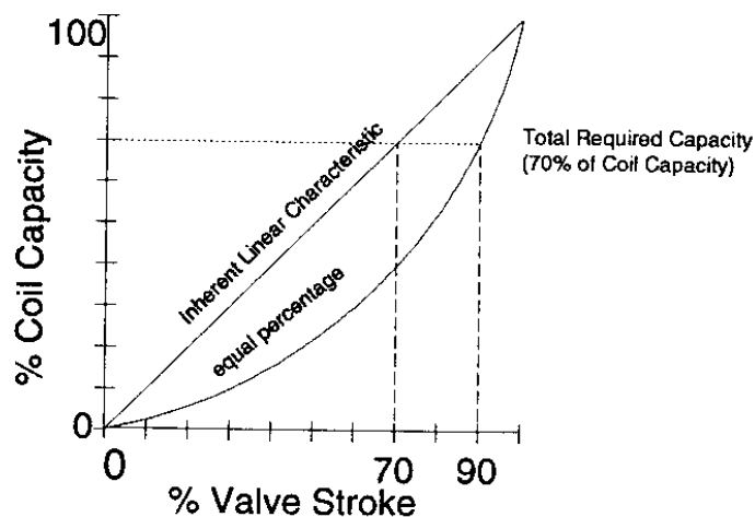
Figure 14: Comparison of Total Valve Stroke Used on Oversized Coils.
