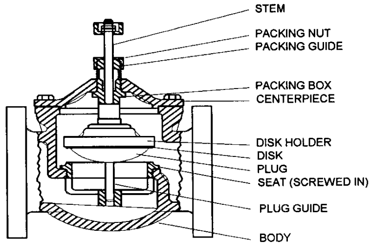
Figure 3: N.O. Cast Iron Flanged Style Valve Body
