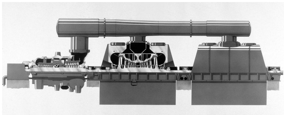
Three-casing, 4-flow ST
