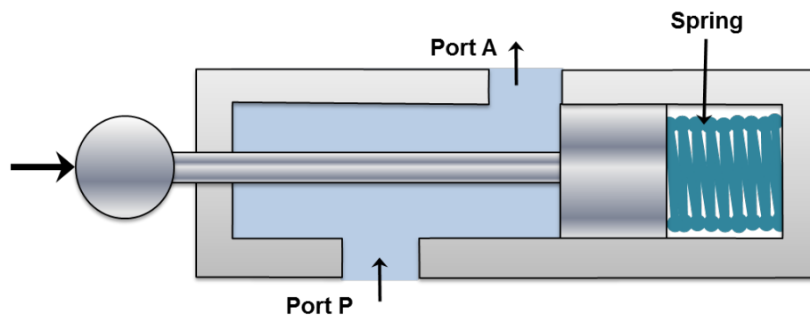
Figure 5.4.6 Valve opened by actuation
