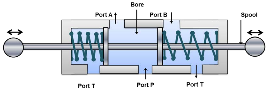
Figure 5.5.2 Three position four way valve: P to A and B to T
