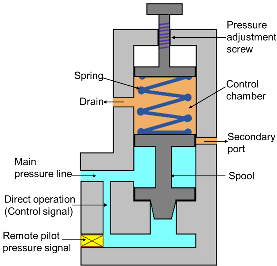
Figure 5.6.3 Sequence valve
