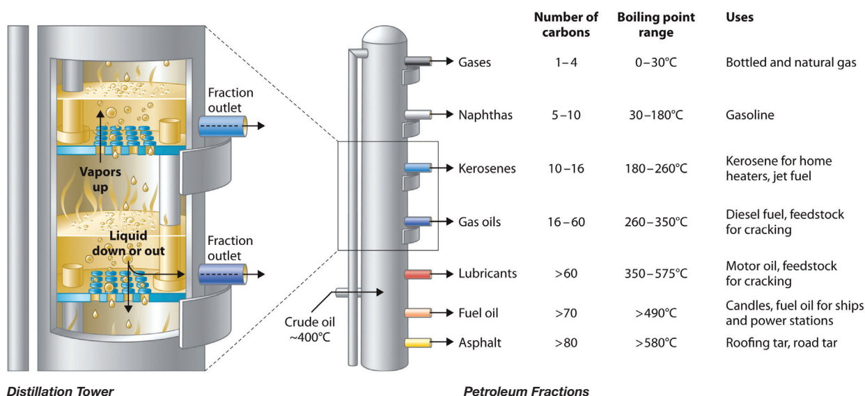
Distillation Tower
