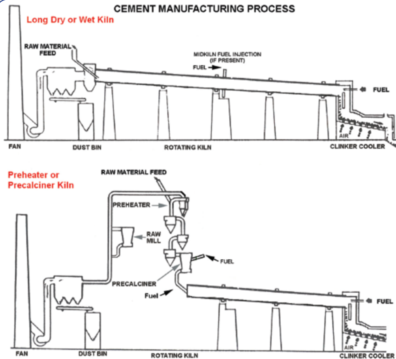
Exhibit 4-1. Cement manufacturing process Source: Portland Cement Association
