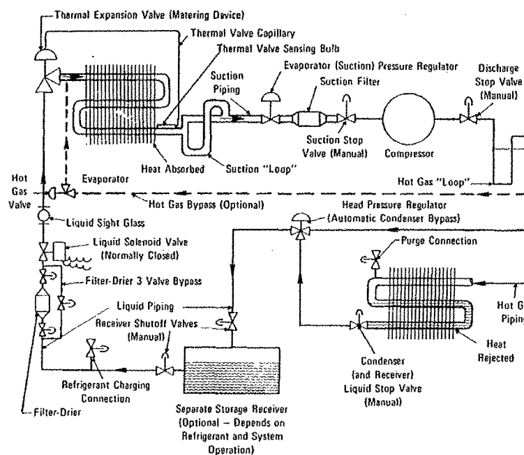
Figure C-17. Flow Components.
