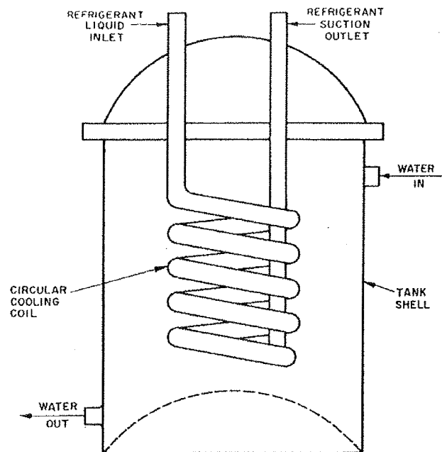
Figure C-22. Shell-and-Coil Cooler.
