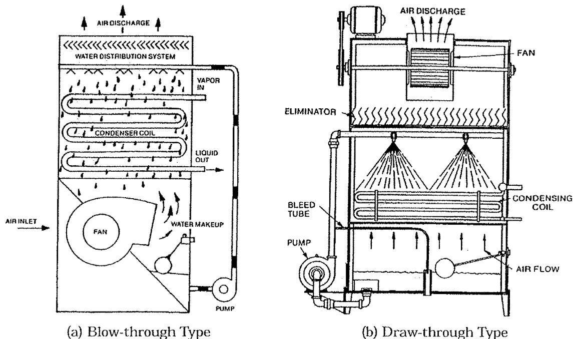
Figure C-16. Evaporative Condensers.
