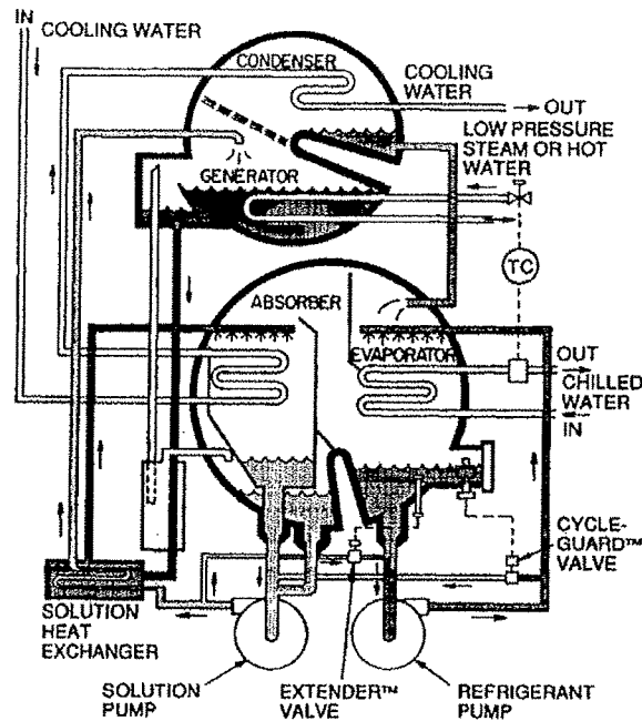
Figure C-7. Absorption Cycle.
