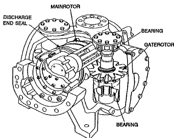
Figure C-4. Single-Screw Compressors.
