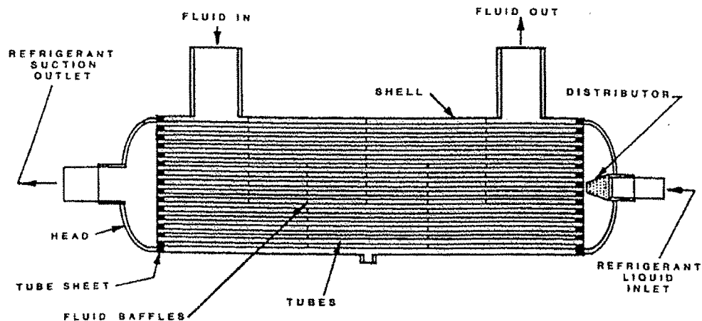
Figure C-19. Direct-Expansion Shell-and-Tube Cooler.
