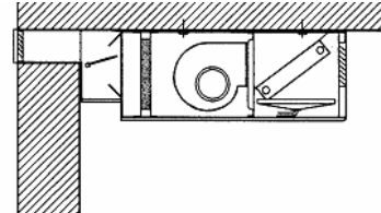
Ceiling fan coil unit with external air intake
