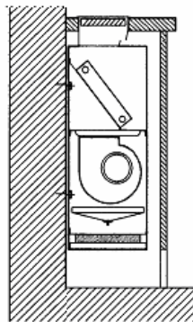
Recessed fan coil unit
