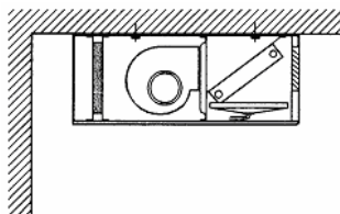
Ceiling fan coil unit
