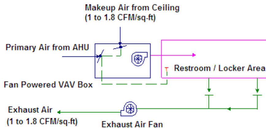
VAV Control for Constant Volume Areas
