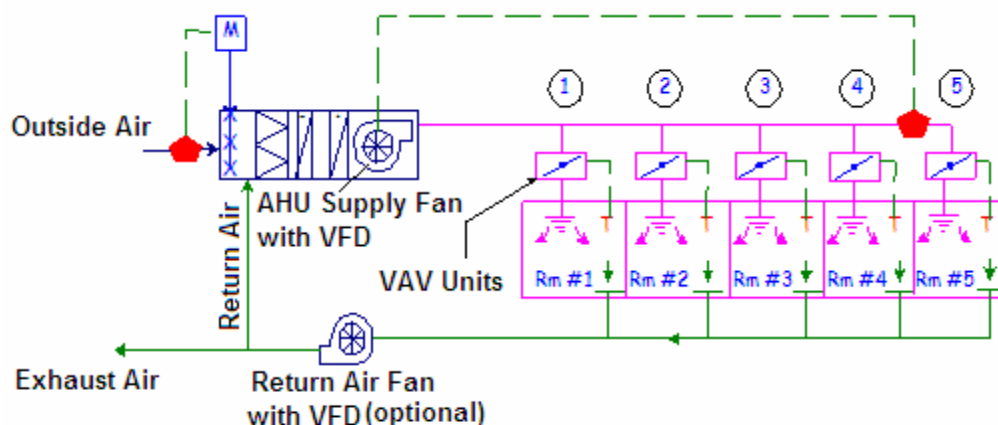
VAV SYSTEM CONTROL SEQUENCE
