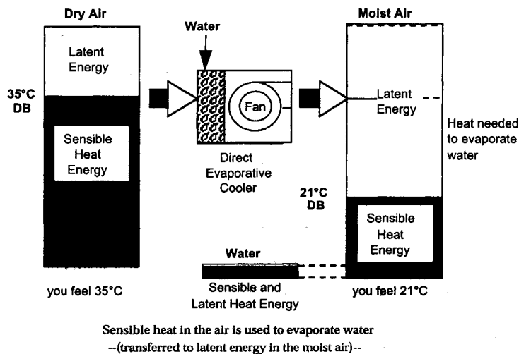
Figure 14: Simplified Evaporative Air-Conditioning Process 14
