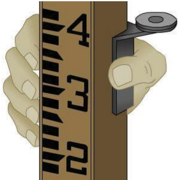
Figure 5-13 - Bull's-eye rod level.
