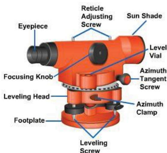
Figure 5-2 - Dummy level.
