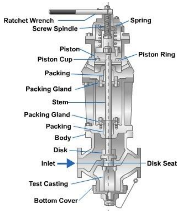
Figure 5-32 – Hydraulic control valve.
