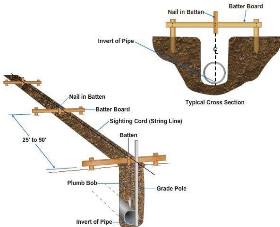
Figure 5-18 - Use of batter boards (with batters) for utility stakeout.
