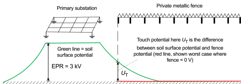
Figure 12 - Third-party fence close to substation
