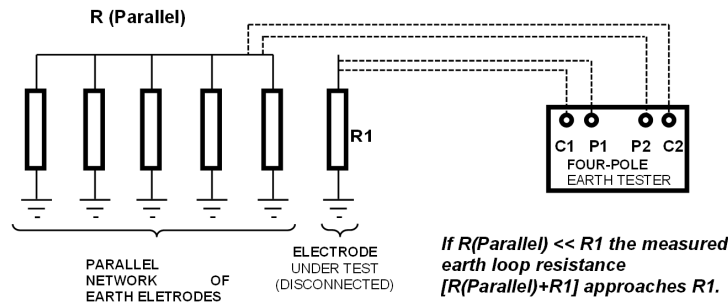
Figure 4 - Earth resistance measurement using the comparative method and a four-pole earth tester (test electrode disconnected)
