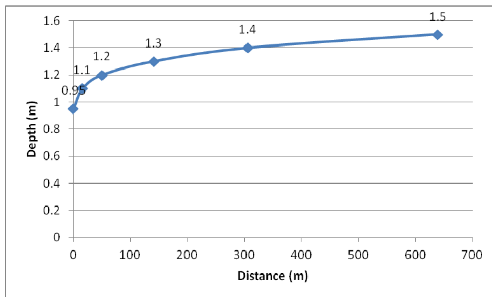
Figure 5.11: Depth Distance Relationship (Draw Down Curve)
