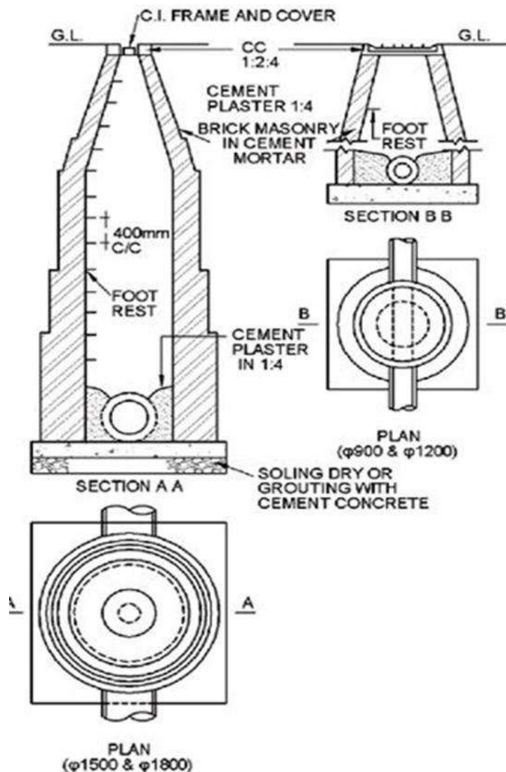
Figure 11.3: Circular Manhole
