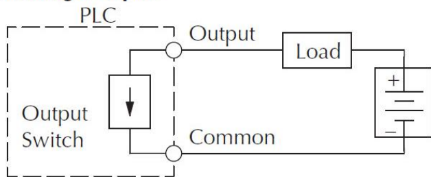
Typical wiring for sinking and sourcing output devices
