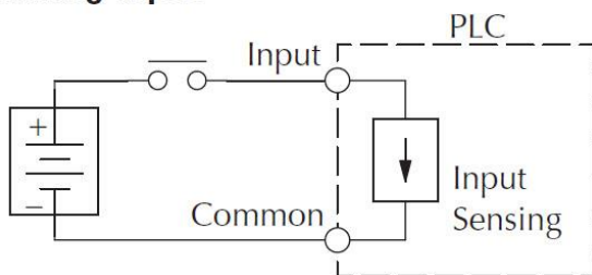
Sinking Input
