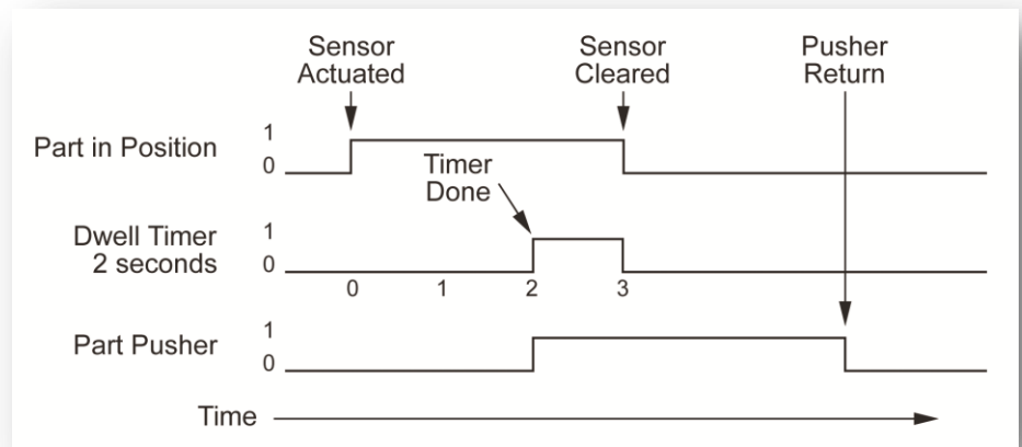
Timing Chart
