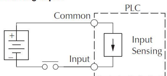
Sourcing Input
