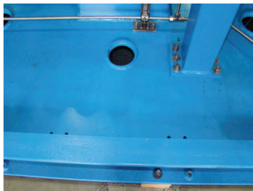
Figure 5. Location of Anchor Bolts on Side Rails of Base Plate.
