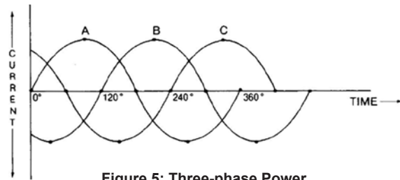
Figure 5: Three-phase Power
