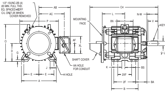
360-5013 Frame (TEFC)
