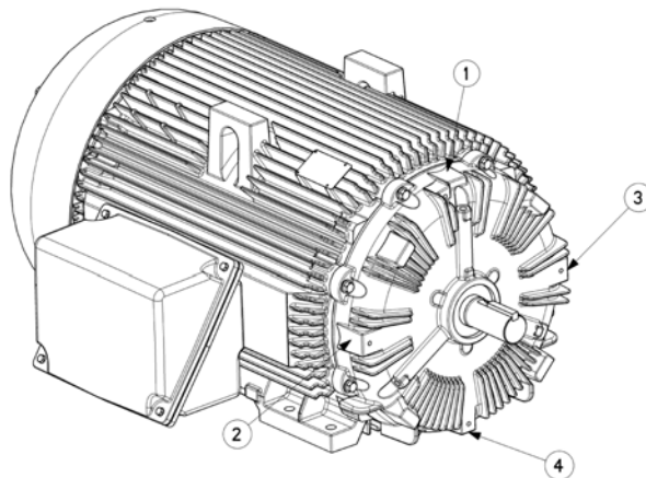
Figure 28: Shows the position of Cast-in Vibration Pads, on Standard XSD Ultra® Motors
