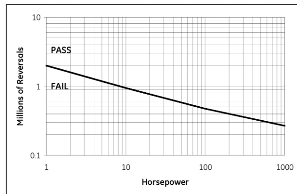
Figure 33: 4-pole GE motor test results data for minimum number of plug-reversals.
