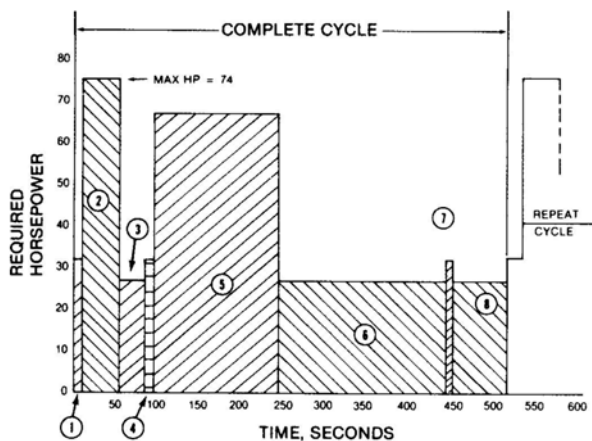
Figure 18: Duty Cycle Calculations
