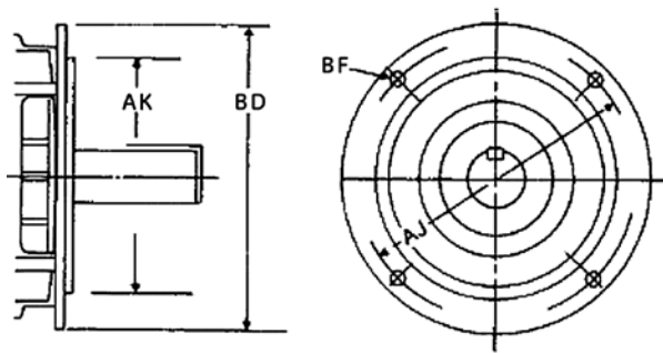
Figure 30: Type D-Flange
