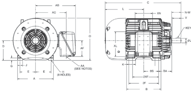
Common Motor Dimensions
