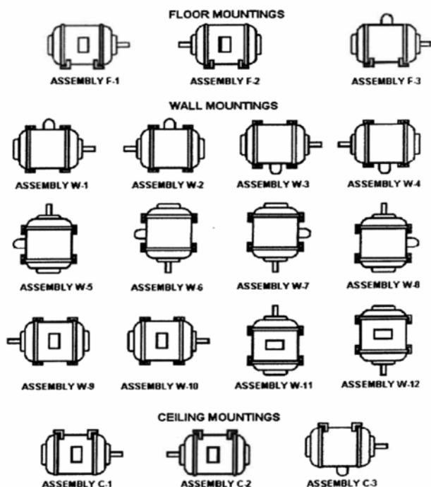
Figure 26: NEMA Mounting
