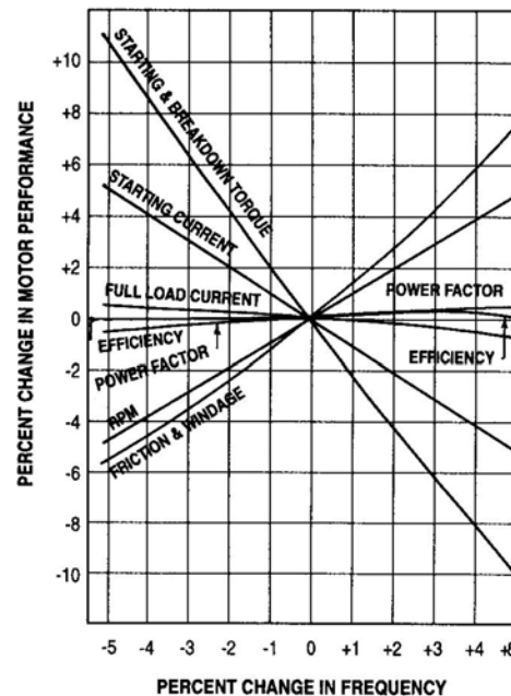
Figure 2: Performance variations with respect to Frequency Variation
