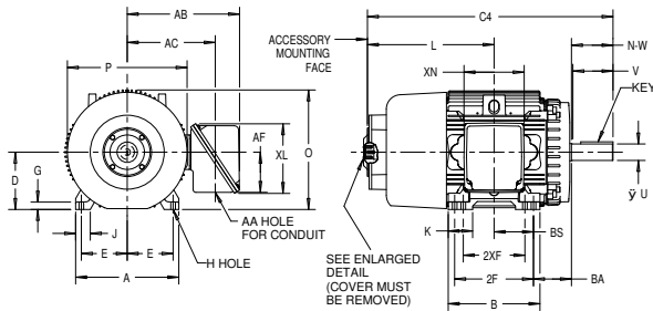
360-5013 Frame (TEFC)
