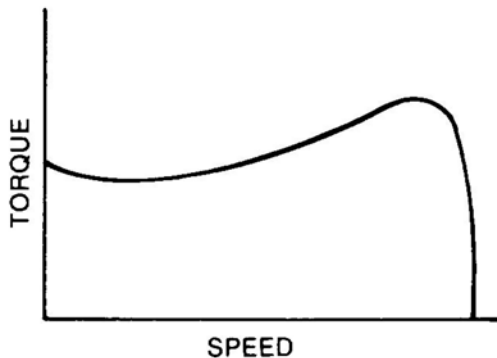
Figure 10: Typical NEMA Design A and B Speed/Torque Curve
