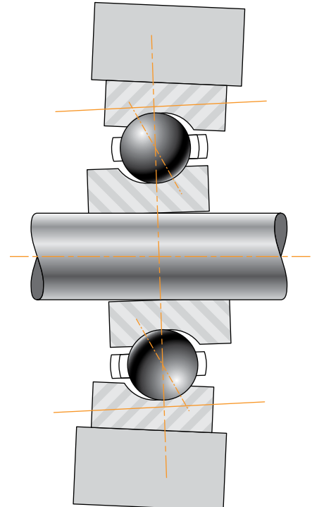
Housing misalignment.
