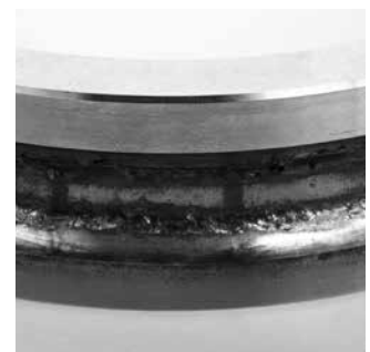
Fatigue spalling from excessive preload.
