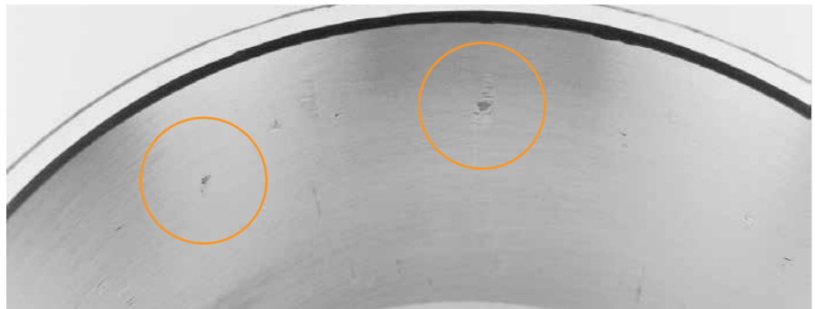
Tapered roller spaced nicking was caused by the roller edges hitting the race during installation. These nicks/dents have raised edges that can lead to excessive noise, vibration or act as points of stress concentration.
