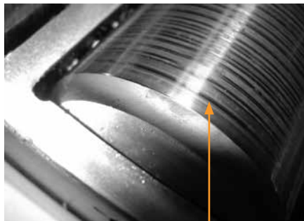
Circumferential grooving on rollers.
