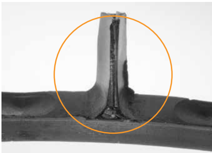
Fine particle contamination entered this spherical roller bearing and generated wear between the cage surfaces, rollers and races.
