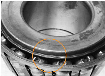
Inner ring rib deformation from excessive heat generation.
