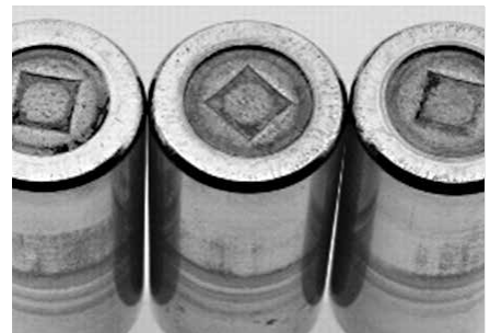
Scoring damage on roller end.
