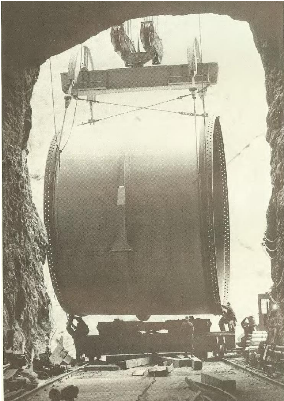
Penstock pipe sections were lowered into the canyon by a 150-ton capacity cableway, then carried into the tunnels on railroad cars.
