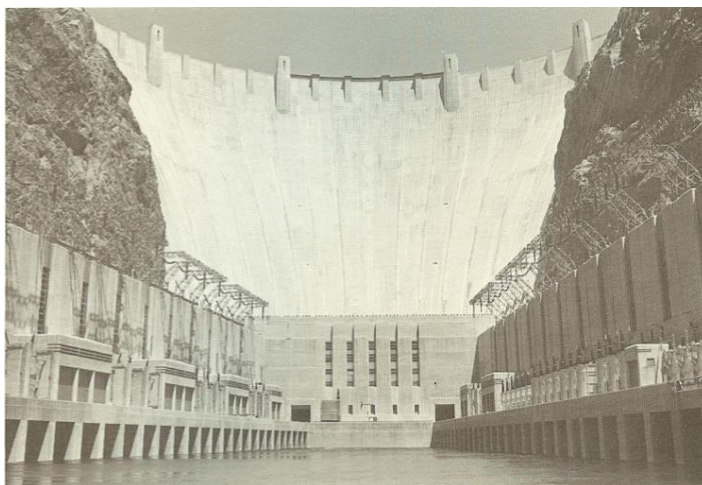
River level view of Hoover Dam. Nevada wing of powerplant is on left, Arizona wing on right. Seven story building at base of dam houses
