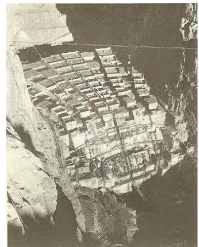
The dam as seen from the control tower of the 150-ton cableway on the Nevada rim of Black Canyon, December 1933.
