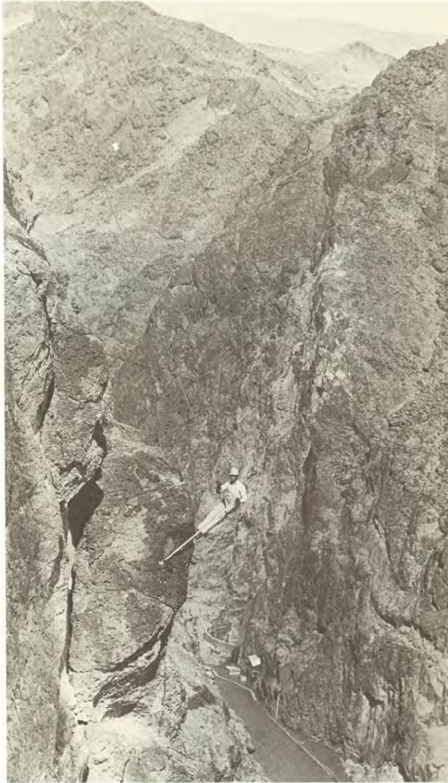
Rigger-rodmen working with topography survey party on Nevada side of Black Canyon at Hoover dam site lowered over canyon rim to provide survey control points which were later used in the design and construction of the dam.
