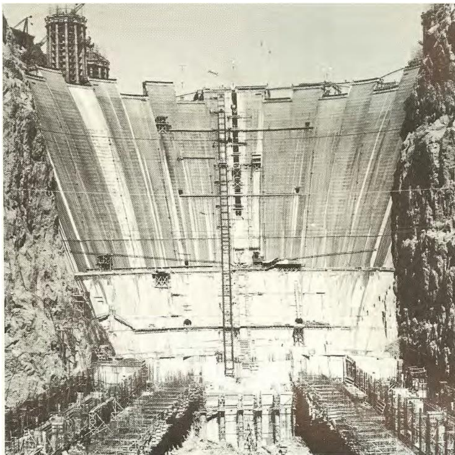
Downstream force of Hoover Dam in February 1934. Dam was built in blocks varying in size from 60 feet square at the upstream side to 25 feet square on the downstream side. Concrete placement in any one block was limited to no more than 5 feet in 72 hours
