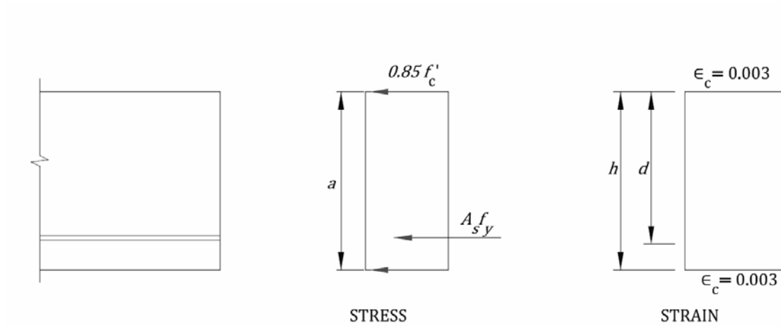
Figure C-5. Stress and Strain under Maximum Axial Load.
