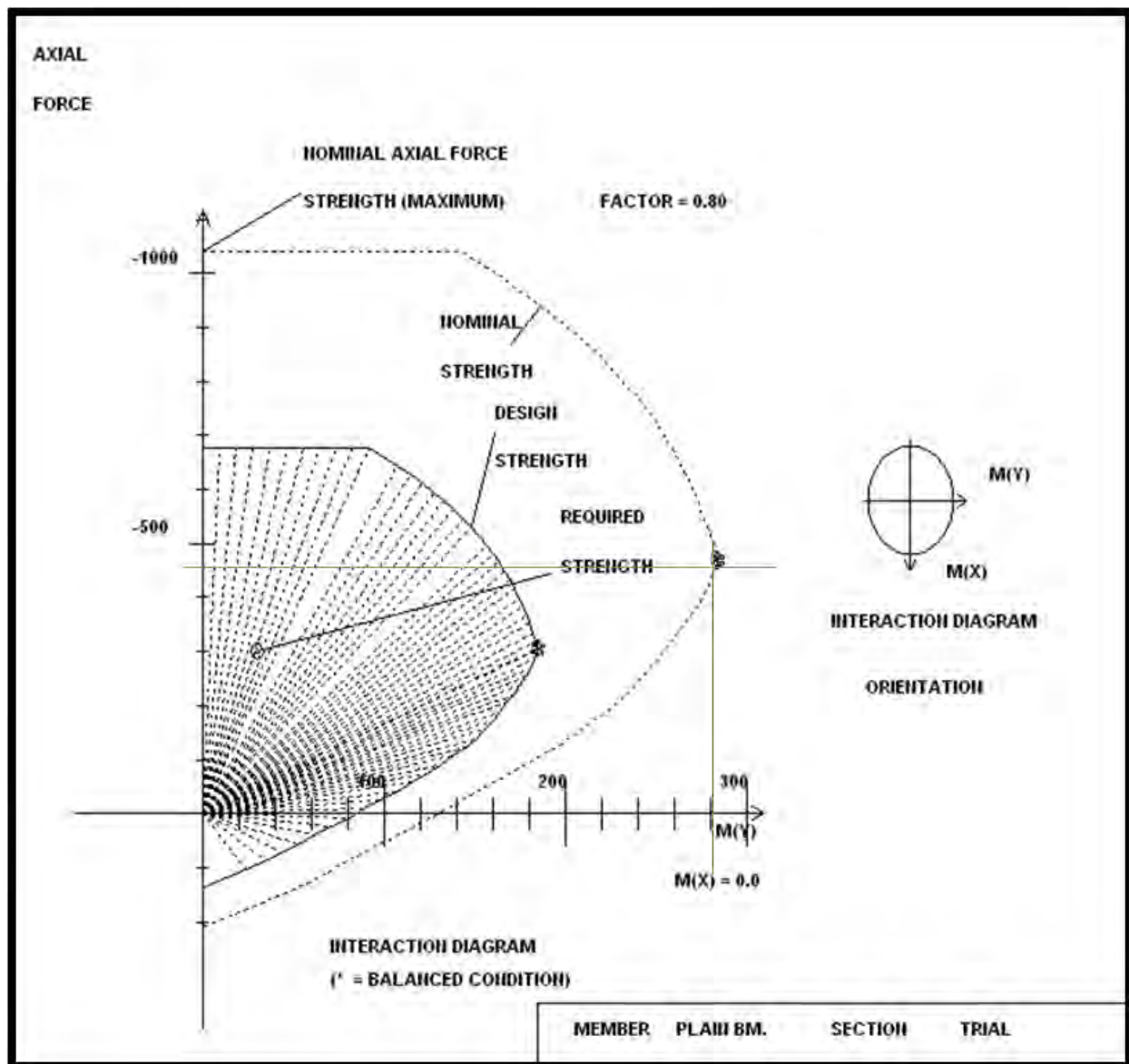
Figure C-14. Nominal Flexural Strength about the Y-Axis
