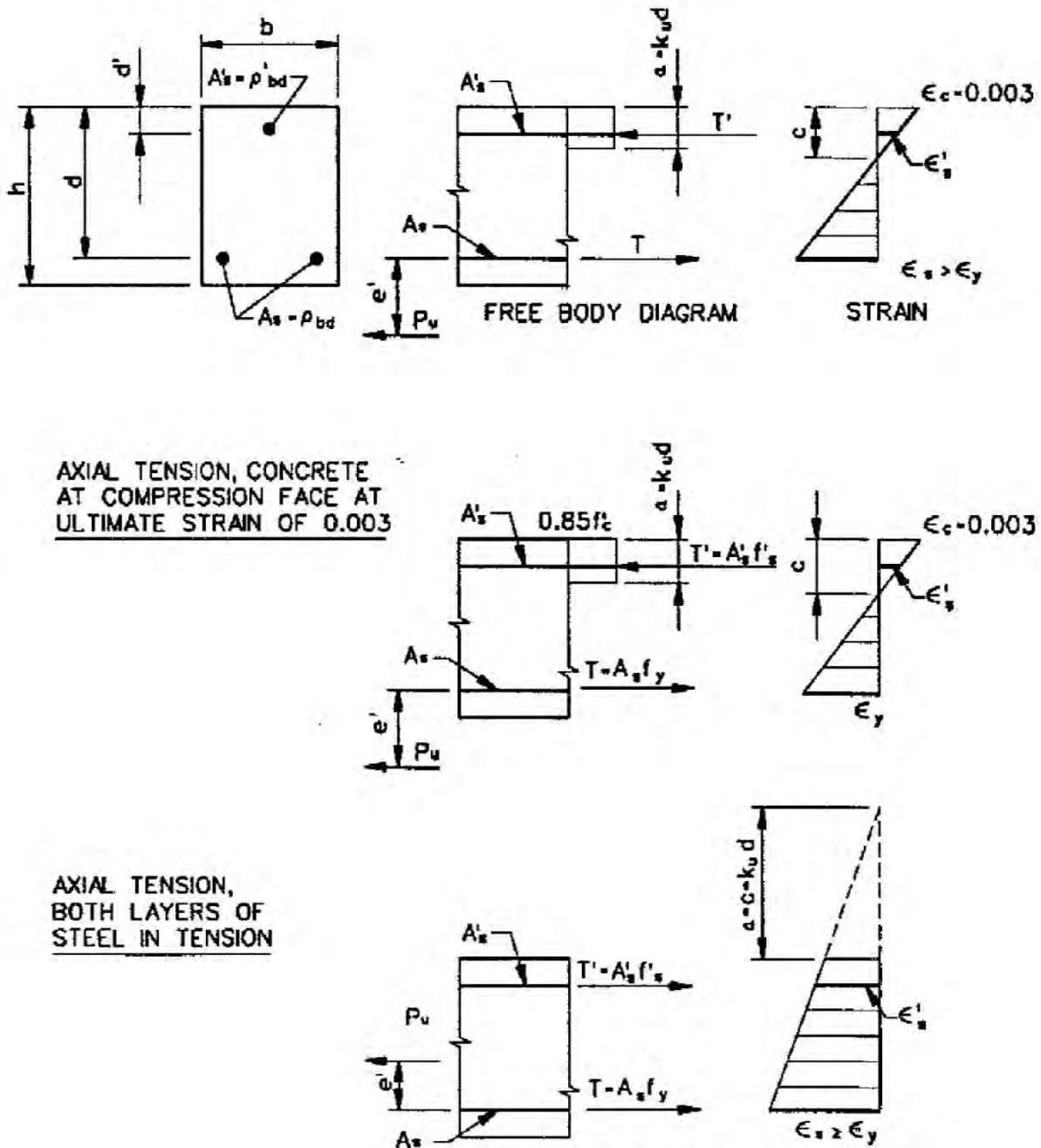
Figure B-3. Axial Tension and Flexure, Double Reinforcement.
