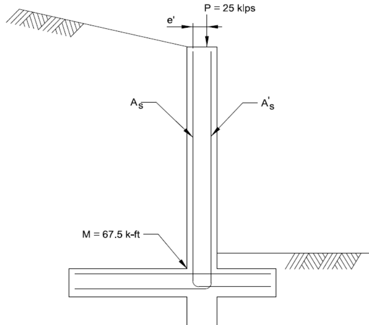
Figure D-5. Retaining Wall with Moment at the Base of Stem plus Axial Load.
