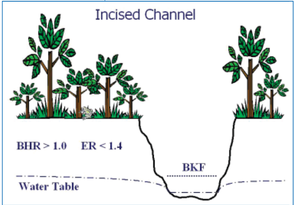
Figure 5.1 Cross section of an incised channel
