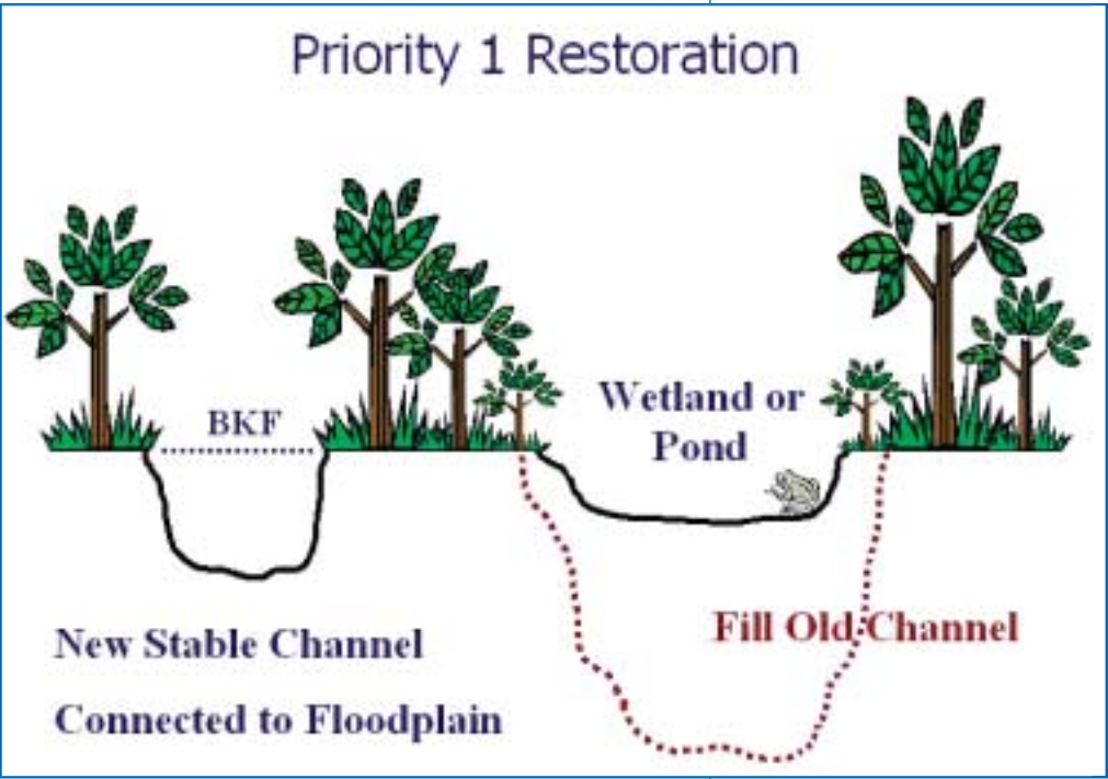
Figure 5.2 Cross section of a Priority 1 restoration project
