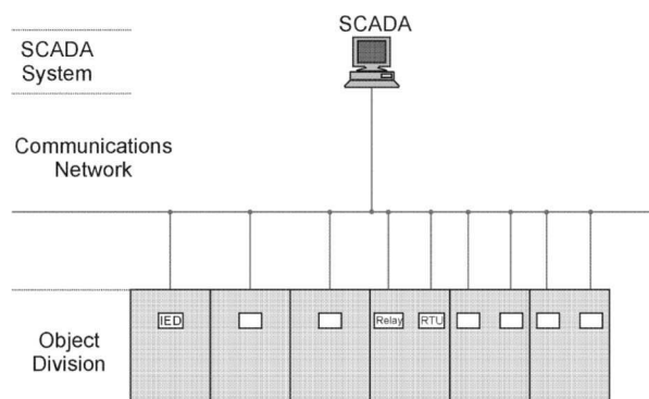
Figure 8.2 Basic architecture of power system automation
