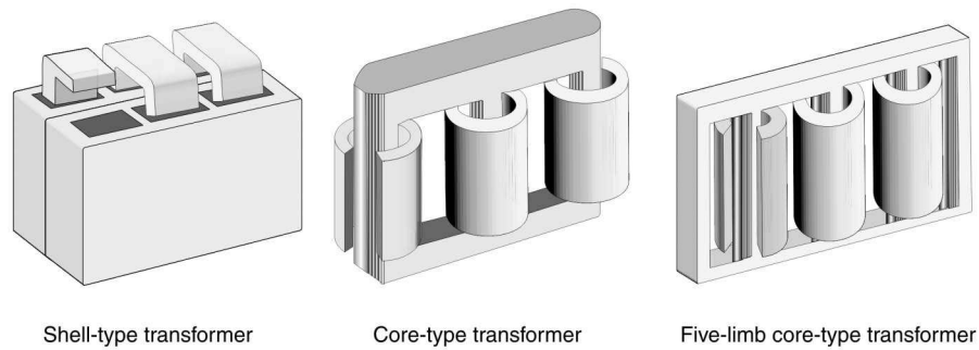
Figure 5.1 Transformer types
