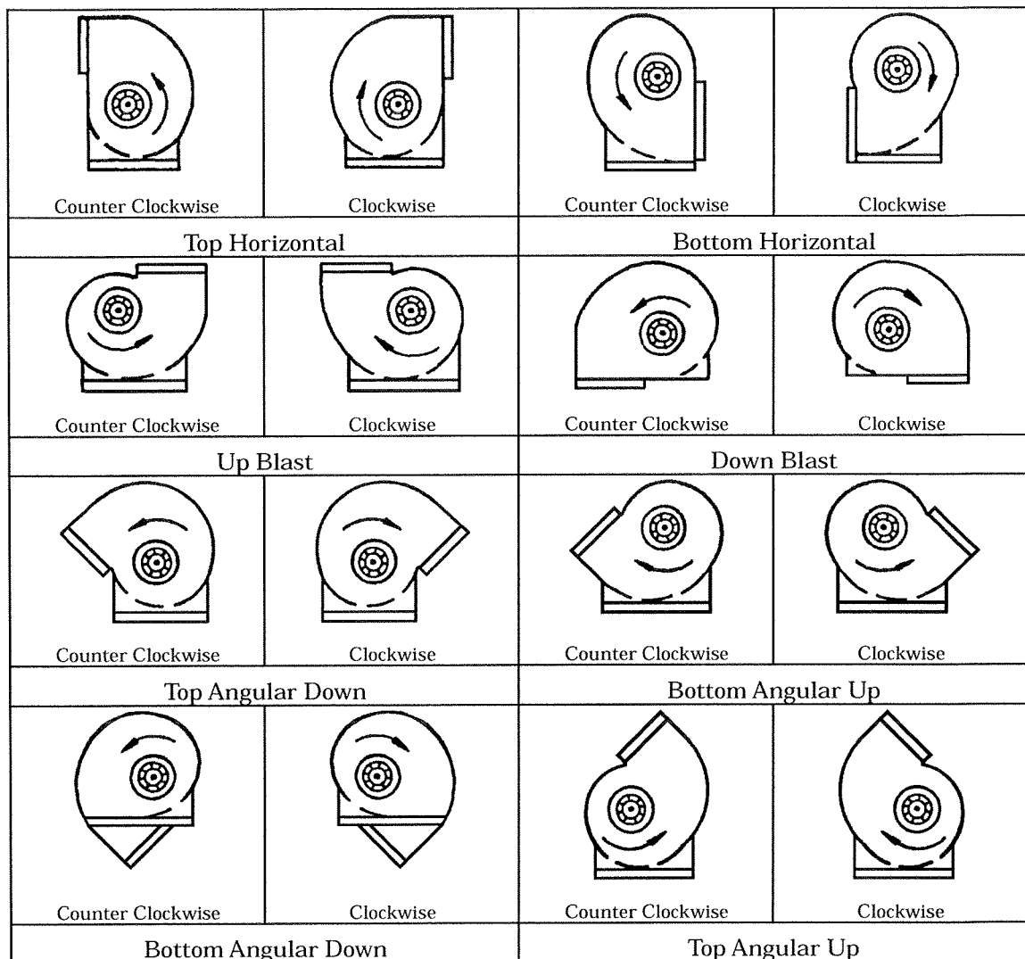
Figure D-25. Direction of Rotation and Discharge.
