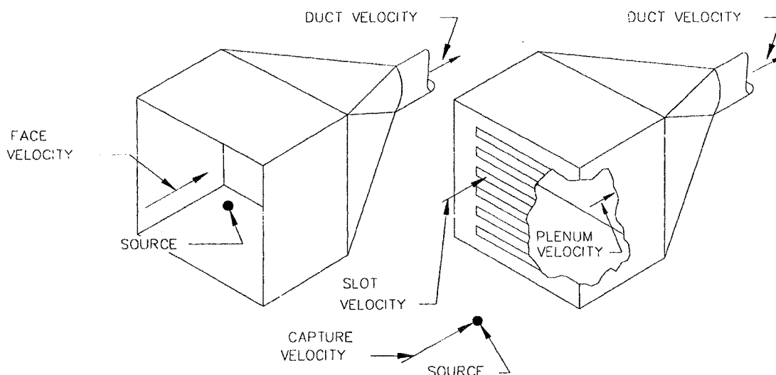
Figure D-37. Basic Exhaust Hood Terms.
