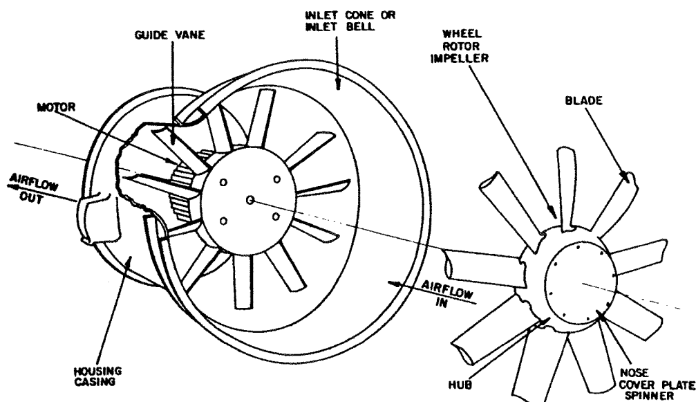
Figure D-15. Axial Fan Components.
