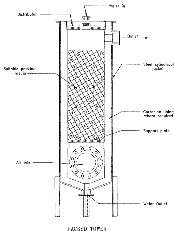
Figure D-33. Packed Tower Collector.
