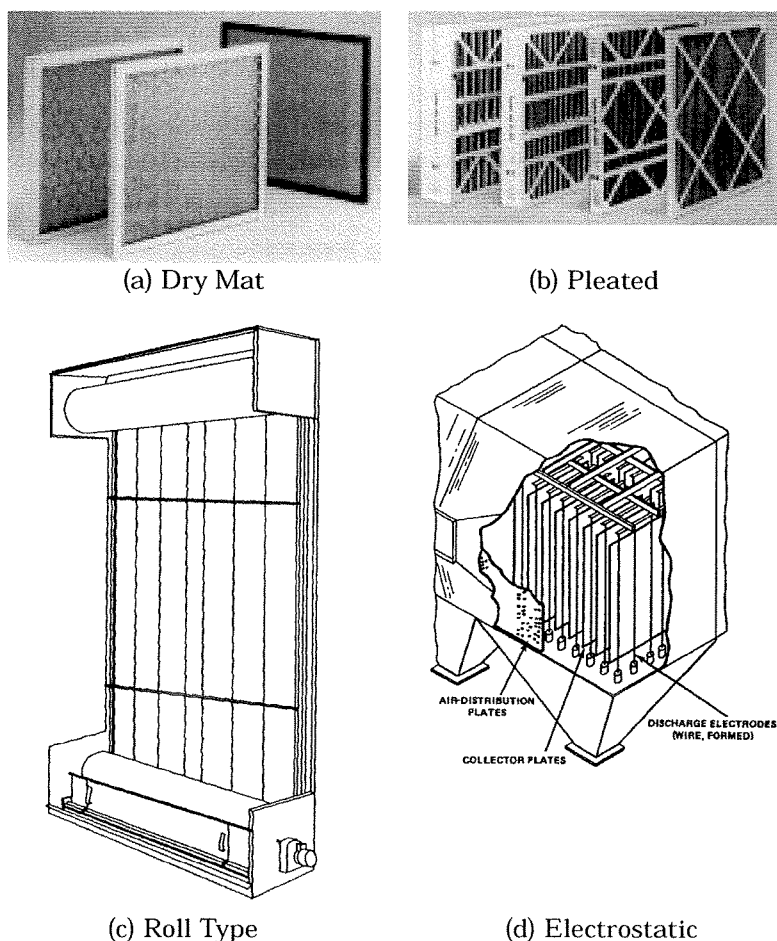
Figure D-29. Air Filter Types.
