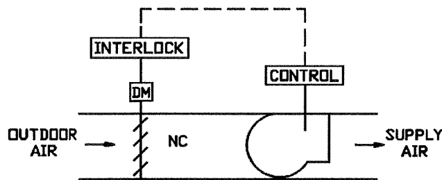
Figure D-42. 100% Outside Air Control.
