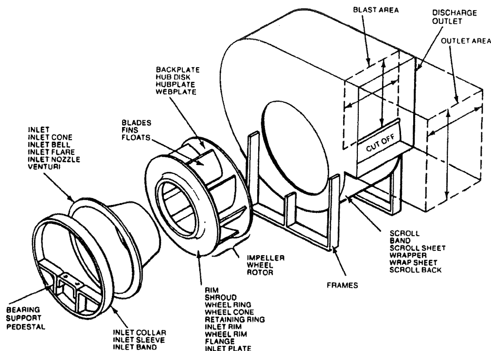
Figure D-10. Centrifugal Fan Components.
