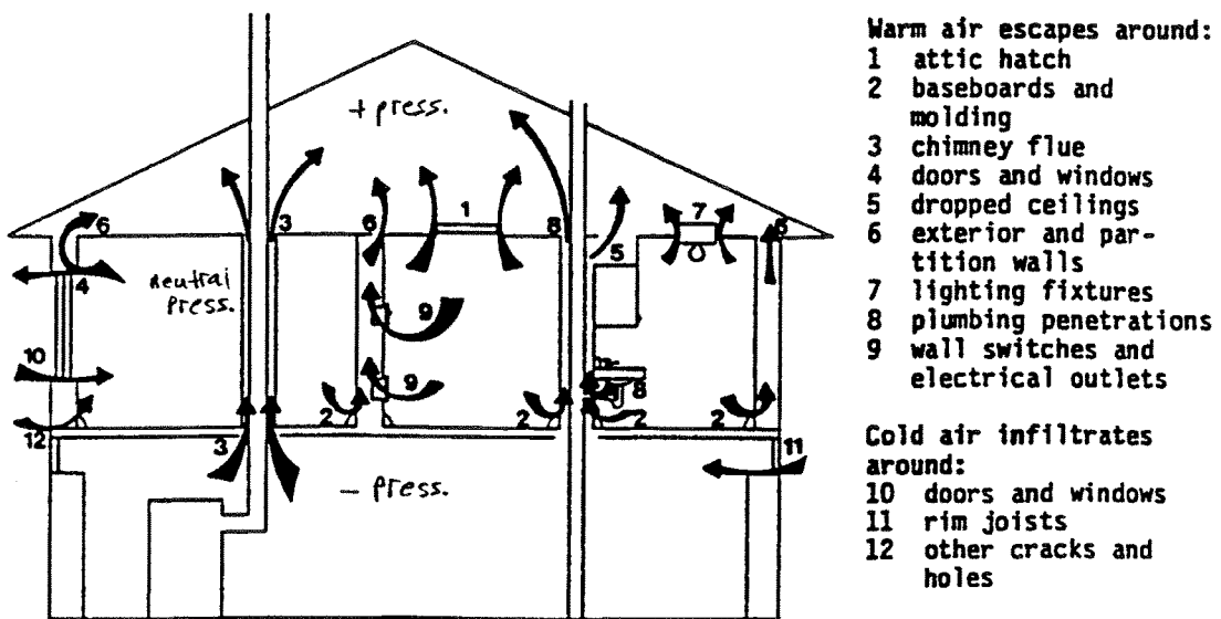
Figure D-5. Natural Air Flow Through a Building.
