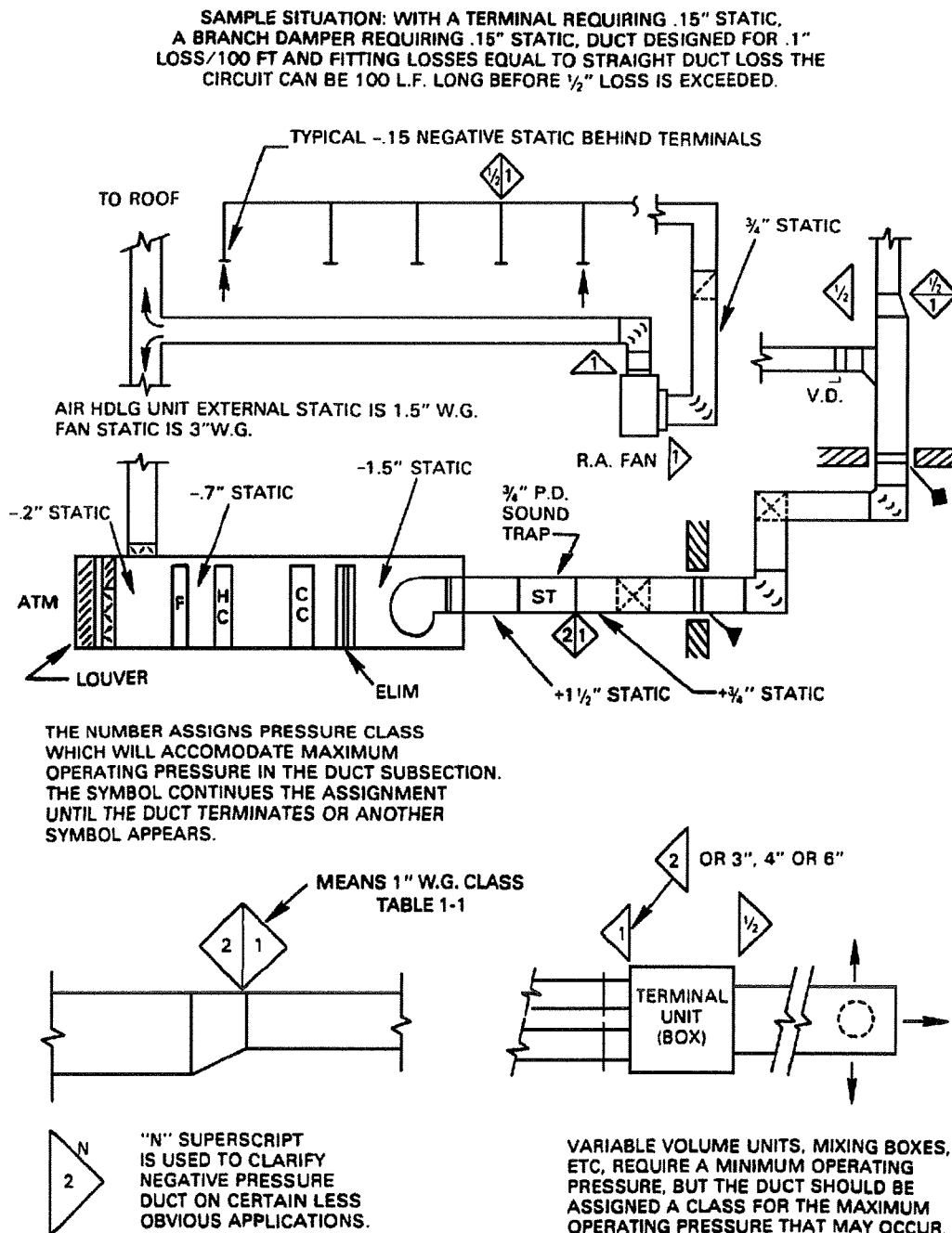
Figure D-28. Duct Pressure Class Designation.
