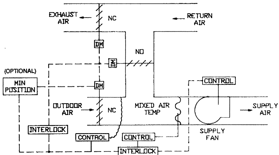
Figure D-43. Economizer Cycle Control.
