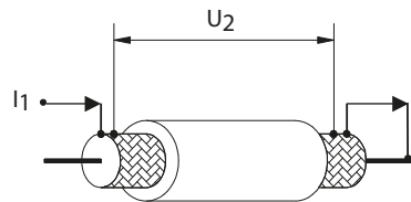
Fig. 6.5 Illustration of transfer impedance
