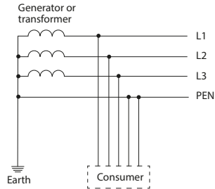
Fig. 7.2 TN-C system: In the entire system, the neutral conductor and the PE conductor are combined in the PEN conductor.
