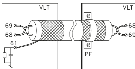
Fig. 6.8 Grounding of the cable shield
