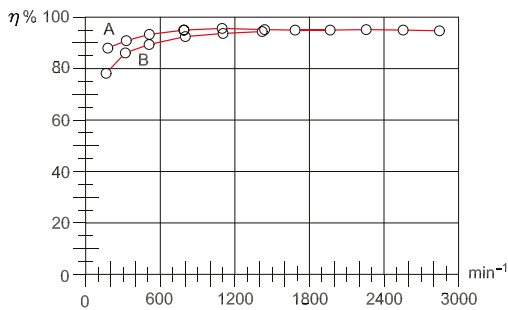
Fig. 5.2 Efficiency example of AC drives
