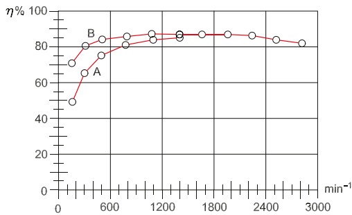
Fig. 5.3 Efficiency example of a 2-pole motor
