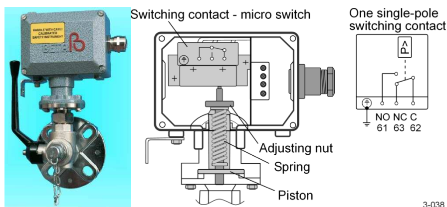
Figure 3.38: Pressure relay
