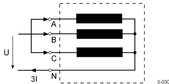
Figure 3.30: Zero-sequence measurement
