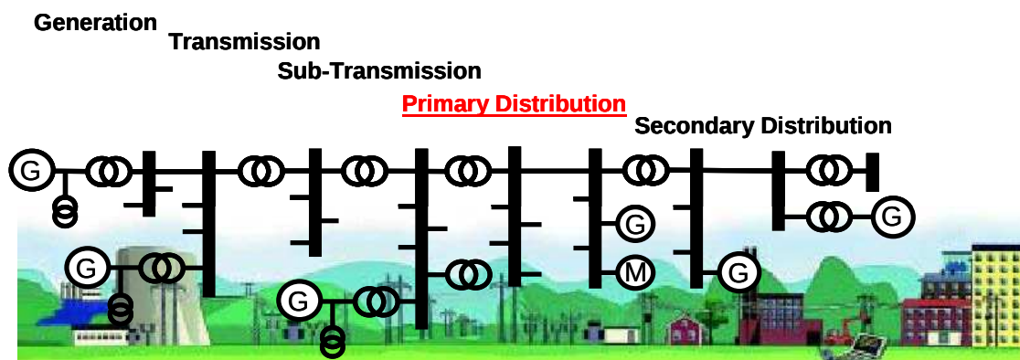
Figure 3.1: Power system
