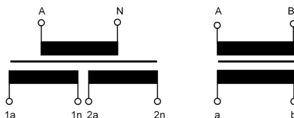
Figure 3.85: Representation of a single-pole (on the left) voltage transformer with two secondary cores and a double-pole (on the right) with one secondary core
