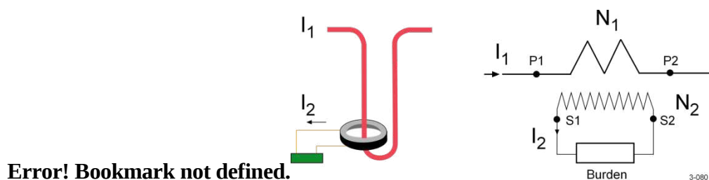
Figure 3.80: Principle presentation of a magnetic current transformer
