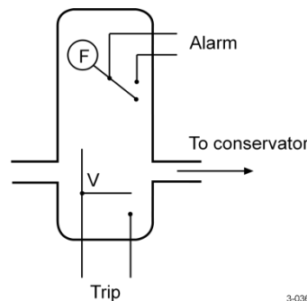
Figure 3.36: Buchholz relay principal construction
