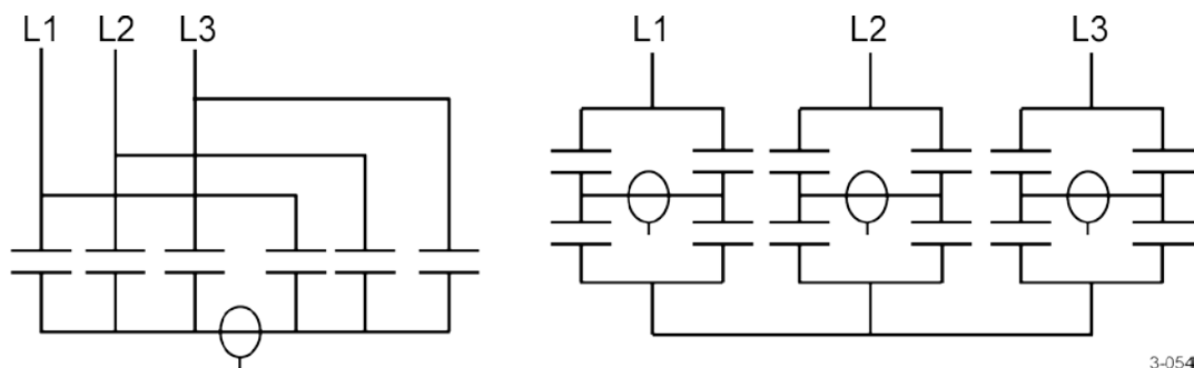
Figure 3.54: A three-phase star (left) and H-bridge-connected (right) capacitor bank with unbalance current measurement
