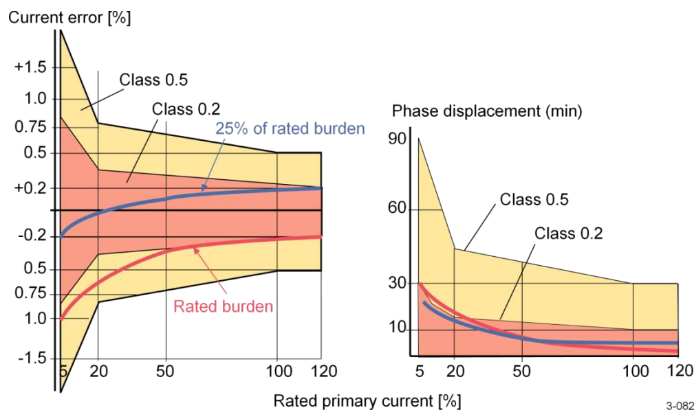
Figure 3.82: Current transformer measurement requirements for classes 0.5 and 0.2 according to IEC standards. Plotted lines show the behavior of the transformer used in above example
