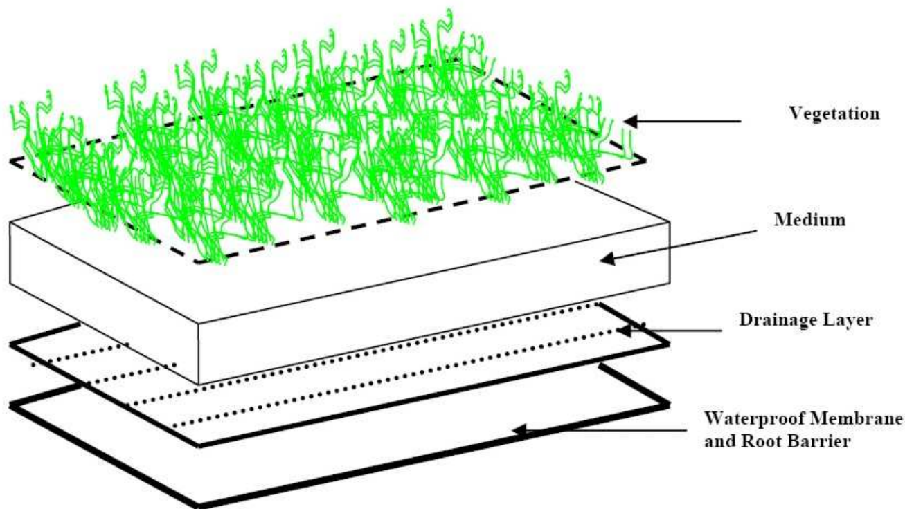
Figure 1-1 Typical cross-section of a green roof system (Berghage et al., 2007)
