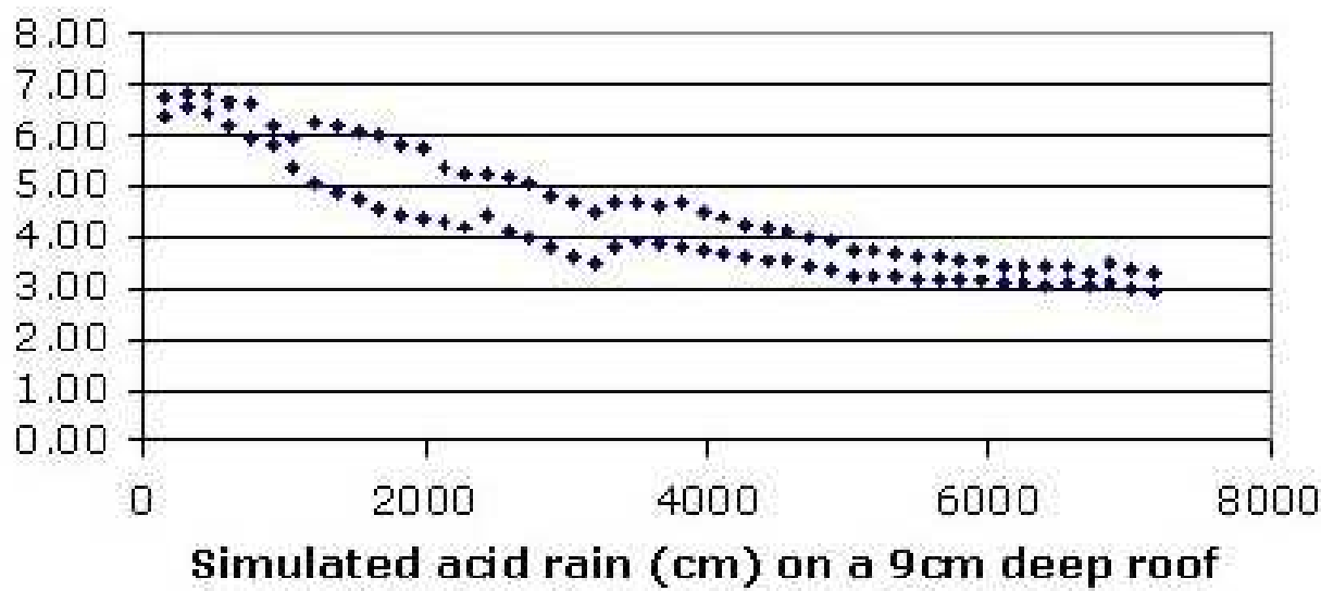
Figure 5-9 Accelerated acid aging trial for clay-based media
