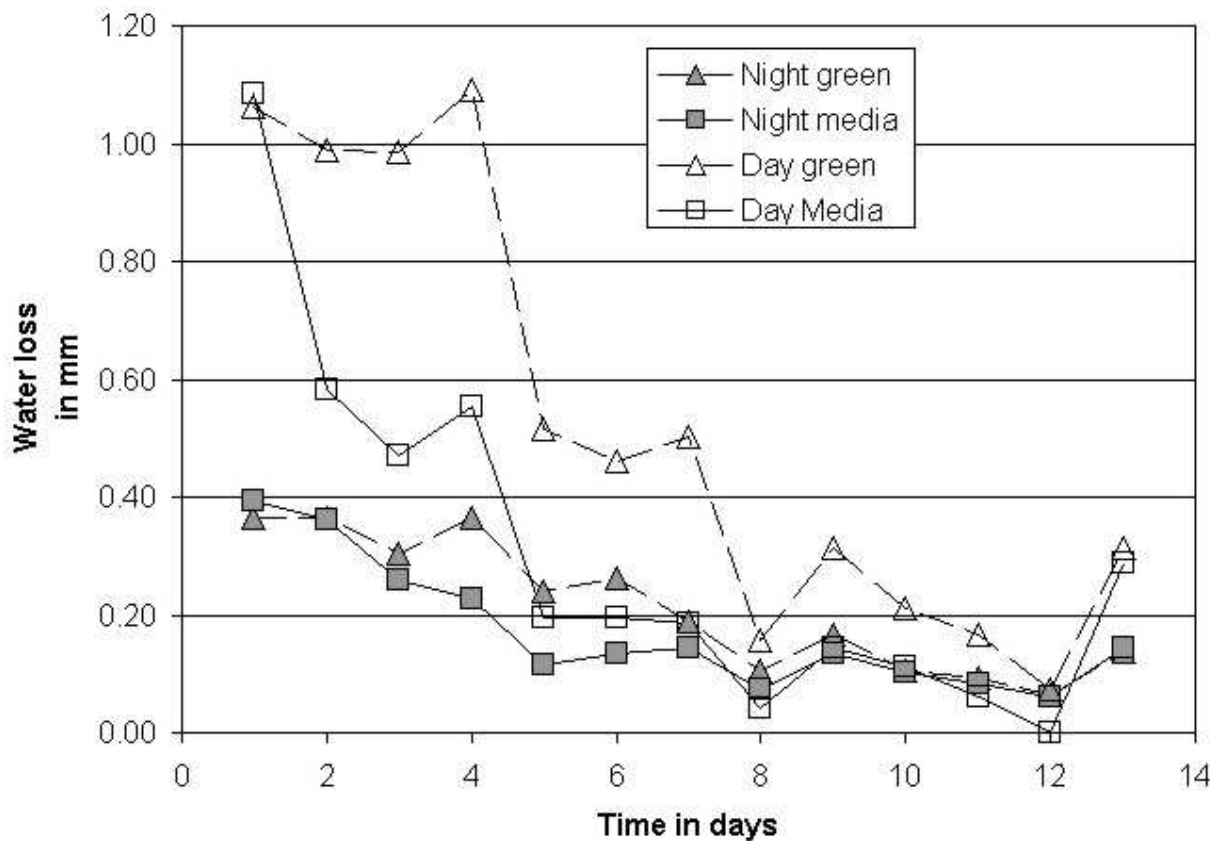
Figure 5-2 Average water loss during the daylight or night from planted and unplanted green roof lysimeter test beds in the fall
