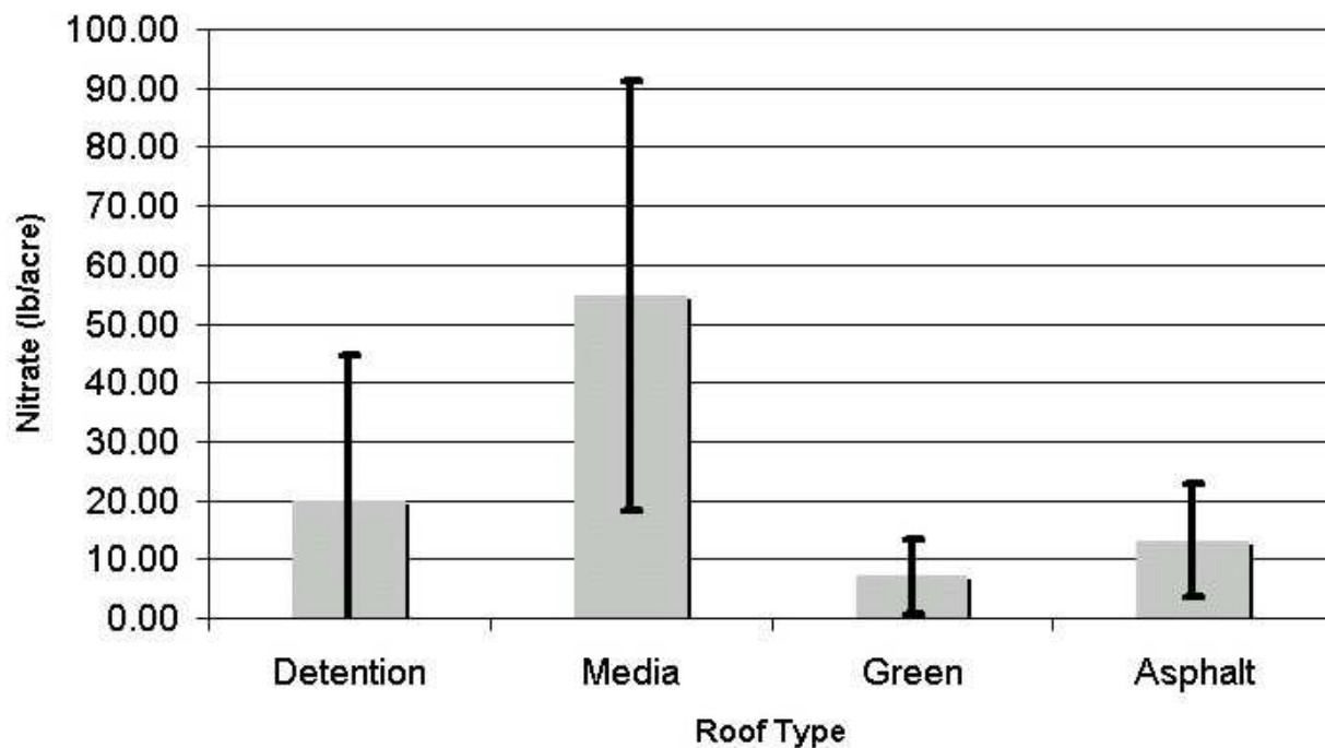
Figure 4-13 Calculated annual loading of nitrate from test roofs
